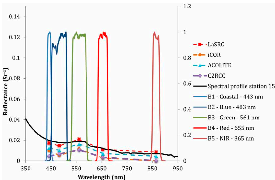
Figure 5. Comparison of atmospheric correction results and field radiometer data for the Laguna Grande lake. The black line depicts the measured water surface reflectance at station 15, which was collected by using the ASD Field-Spec 4 spectroradiometer.
