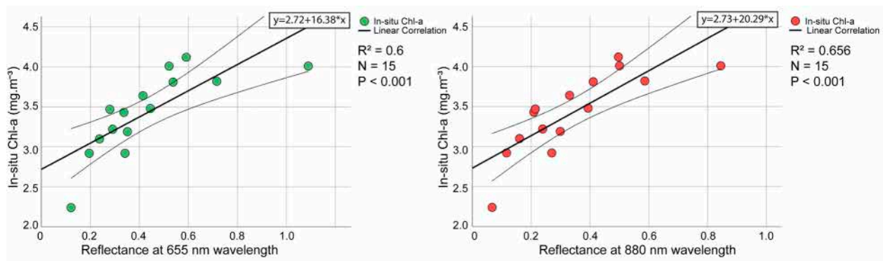
Figure 7. Relationship between Chl-a concentration and reflectance at wavelengths of 655 nm and 880 nm.
