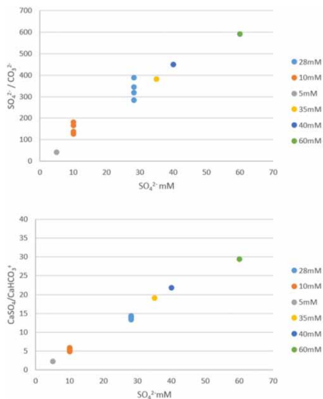
Figure D1. Geochemical modeling results showing \text{SO}_4^{2-} / \text{CO}_3^{2-} ratio and \text{CaSO}_4 / \text{CaHCO}_3 ratio in a solution as a function of total sulfate concentration in a solution (dot colors indicate each sulfate concentration). Each point corresponds to a different computational run, for samples where DIC and pH were measured and were used as constraints to the model. Both ratios increase linearly to a slight inflection point at 60 mM, but no plateau is seen between 28 and 60 mM.
