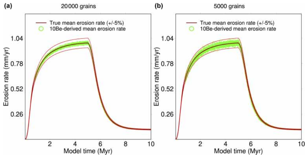
Figure 5. Effect of seeding the model with a different number of grains on the mean ^{10}\text{Be} -derived erosion rate calculated from the mean ^{10}\text{Be} concentration of outgoing grains. Panel (a) represents 20 000 grains (two per cell on average). Panel (b) represents 5 000 grains (one out of every two cells on average).
