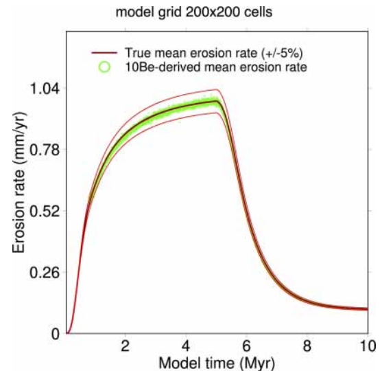
Figure 8. Effect of multiplying the model grid size by four on the mean ^{10}\text{Be} -derived erosion rate calculated from the mean ^{10}\text{Be} concentration of outgoing grains. The number of grains is also multiplied by four to have one grain per cell on average as in the reference simulation.
