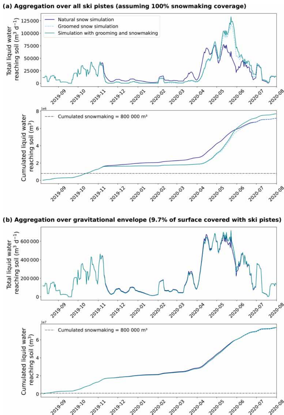
Figure 5. Aggregation over all ski pistes (a) and for the entire ski resort gravitational envelope (b) of the daily liquid water reaching the soil and cumulative liquid water reaching soil, respectively, for the natural snow (solid blue line), grooming snow on ski pistes (dashed green line) and grooming and snowmaking on ski pistes (solid green line).
