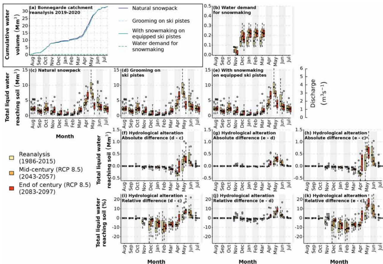
Figure 9. Overview of the hydrological alteration due to grooming and snowmaking in the Bonnegarde catchment, based on the SAFRAN-Crocus simulations. Simulations take into account either natural snow only (c), grooming on ski pistes and natural snow around the pistes (d), and grooming on ski pistes and snowmaking on the parts of the ski pistes equipped with snowmaking equipment, and natural snow around the pistes (e). Here we do not take into account the water abstraction used for snowmaking (similar to Fig. 5). Panel (a) shows the aggregated total water reaching soil for the whole catchment for the hydrological year 2019–2020 (similar to Fig. 5). Panels (b) to (k) show various components and visualizations of the local hydrological cycle under past climate conditions (reanalysis, 1986–2015) and using climate projections (RCP8.5, centered on 2050 (2043–2057) and 2090 (2083–2097)). Panels (c) to (e) show the distribution of monthly aggregations of total water reaching soil under these three climate contexts. Panel (b) shows the cumulative water demand for snowmaking under these three climate contexts. Panels (f) to (h) show the hydrological alteration, here computed as the difference between monthly aggregated total water reaching soil between different configurations and with various references (natural snow only, or taking into account grooming on ski pistes). Panels (i) to (k) show the relative alteration, i.e. same as panels (f) to (h) but relative to the corresponding reference values.
