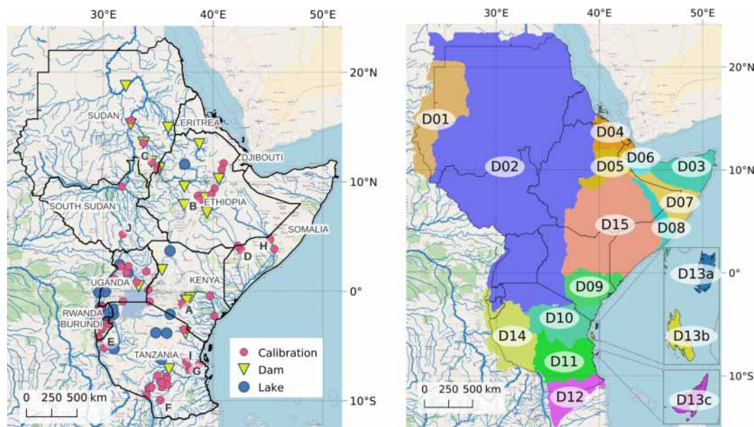
Figure 1. GHA region with dams, lakes, and calibration stations included in the model (left). The 17 simulation domains implemented (right). © OpenStreetMap contributors 2023. Distributed under the Open Data Commons Open Database License (ODbL) v1.0.
