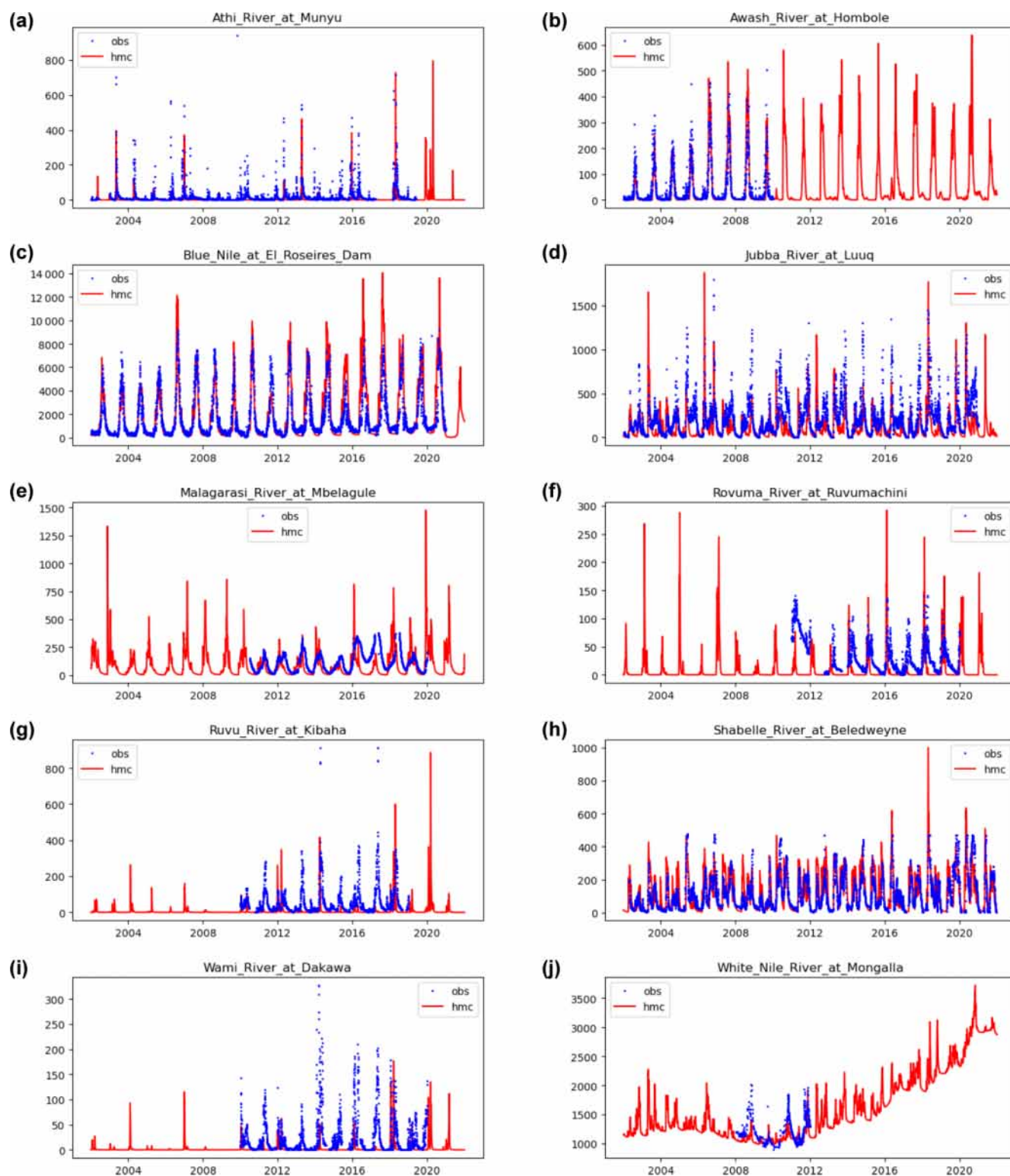
Figure 3. Comparison of simulated versus available observed discharges at 10 stations sampled from all 8 validation domains for the period 2002–2021.
