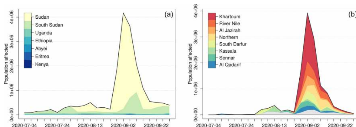
Figure 6. The 5 d forecast of population affected in the Nile Basin for the period July–September 2020 from FPEA. Country totals (a) and aggregations for the Sudanese states (b).
