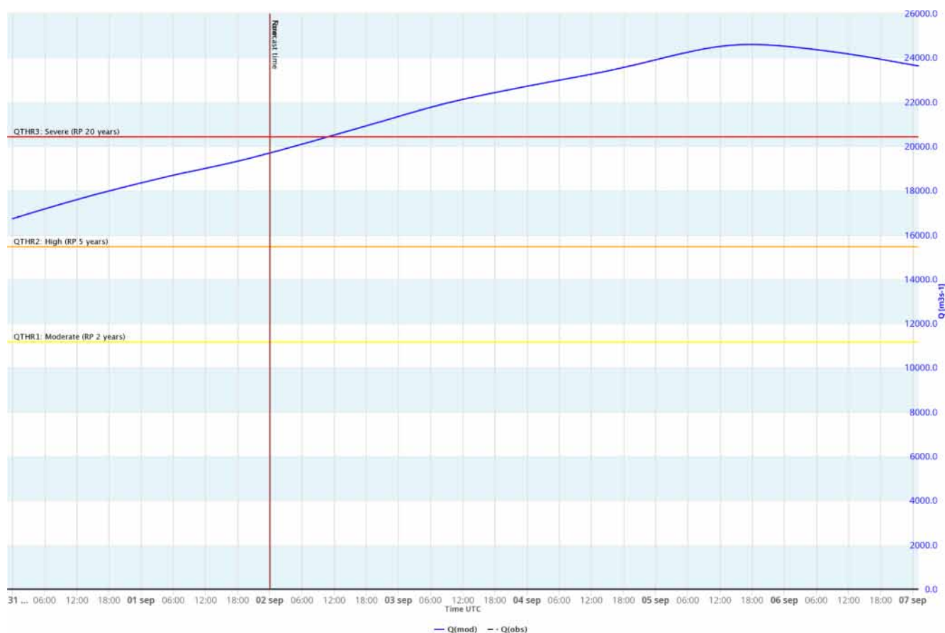
Figure E2. Flood-PROOFS East Africa forecast run of 2 September 2020, 00:00 UTC. Reporting point in the Blue Nile at Khartoum Manshia Bridge. Peak flow is forecast in the evening of 5 September. Maximum water level was observed on 7 September 2020.
