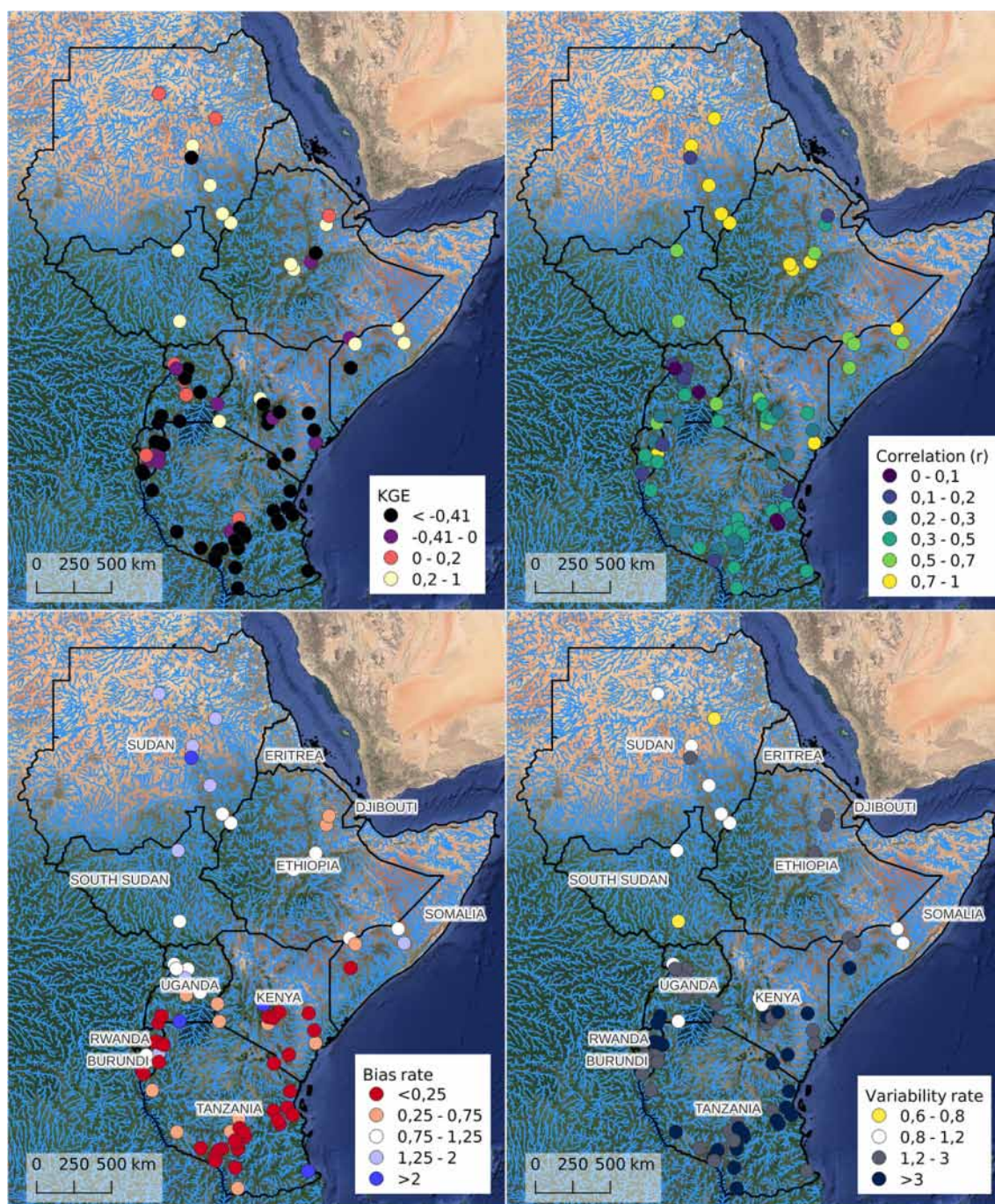
Figure 2. Validation skills at 78 river gauges: KGE and its decomposition term correlation ( r ), bias rate, and variability rate. Numeric values are reported in the Supplement. Map data: © Google 2019.
