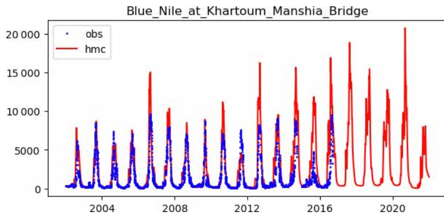
Figure E1. Comparison of simulated versus available observed discharges in the Blue Nile at Khartoum Manshia Bridge. The September 2020 flow peak is the largest in the long-term simulation.
