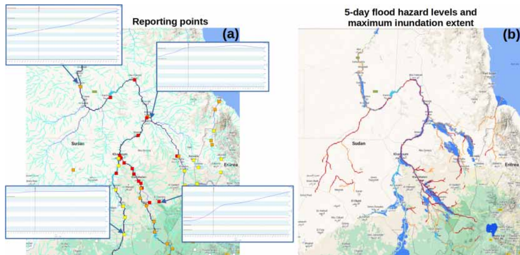
Figure 4. FPEA forecast on 2 September 2020 from the myDEWETRA web platform. (a) Reporting points and 5 d discharge forecast at four sample points and (b) 5 d forecast of flood hazard levels and maximum inundation extent. Map data: © Google 2019.
