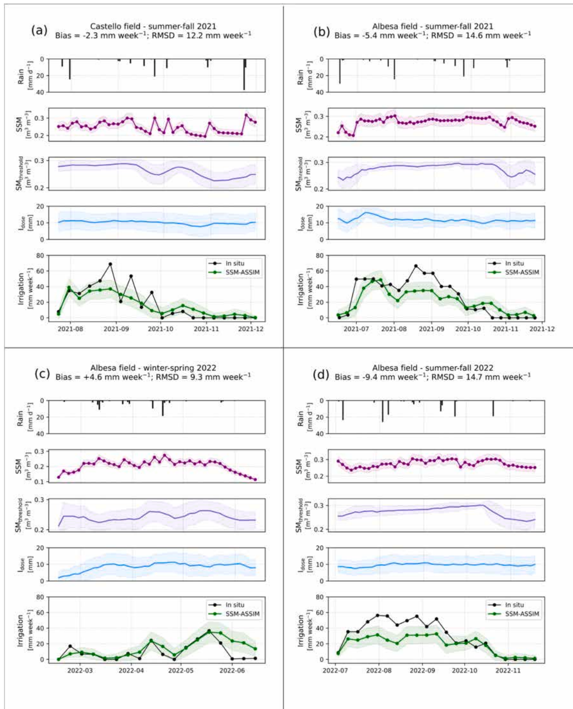
Fig. 6. Daily rainfall (black bars), in situ SSM every three days (purple line), daily SM_{threshold} (dark blue line), daily I_{dose} (light blue line), and weekly irrigation retrieved with the SSM-ASSIM approach (green line) and weekly in situ irrigation (black line), for Castello summer-fall 2021 (a), Albesa summer-fall 2021 (b), Albesa winter-spring 2022 (c), and Albesa summer-fall 2022 (d) separately.
