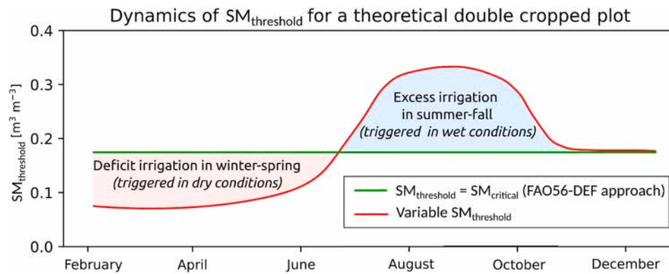
Fig. 3. Schematic dynamics of SM_{threshold} for a hypothetical double-cropped plot for an ideal (FAO56-DEF; green line) and real (red line) case. The red shaded area represents deficit irrigation due to SM_{threshold} values lower than SM_{critical} (during winter-spring in this theoretical example) and the blue shaded area represents excess irrigation due to SM_{threshold} values higher than SM_{critical} (during summer-fall in this theoretical example).
