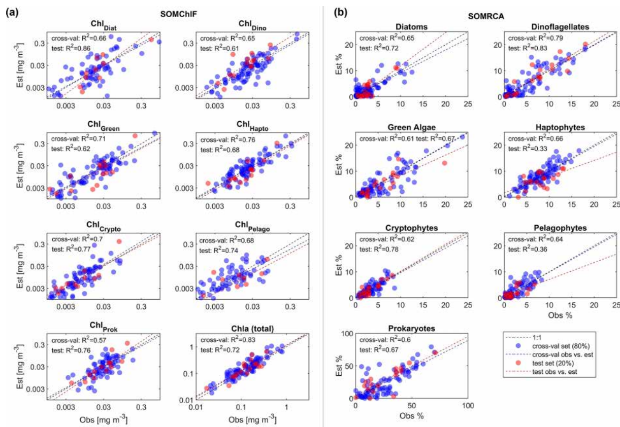
Figure 5. Results of the two-step cross-validation (blue) and test (red) procedures for SOMChIF (a) and SOMRCA (b) with the chosen best combination of satellite parameters and a SOM grid, respectively, of 242 and 222 neurons. From the initial dataset consisting of 145 observations, two sets were split: 80 % to be used in a one-leave-out cross-validation procedure and 20 % as an independent test. For the cross-validation, each observation among the 115 observations was used iteratively as a training set and as a test set until all observations served as tests (blue dots). This procedure was used to identify the best satellite combination and SOM grid size. Finally, the remaining 30 observations were used as a test to evaluate the generalization capacity of the SOM with the chosen configuration (red dots). One should note that, for SOMChIF, the R^2 was calculated using log-transformed Chl a values. For complete evaluation metrics refer to Table 3.
