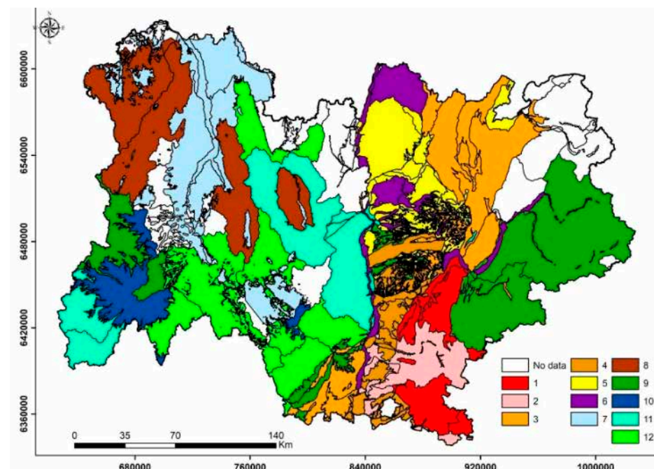
Figure 5. Distribution of homogeneous GWB groups across the Auvergne-Rhône-Alpes region. The GWBs left in blank are those for which the quantity of data was insufficient within the full matrix.
