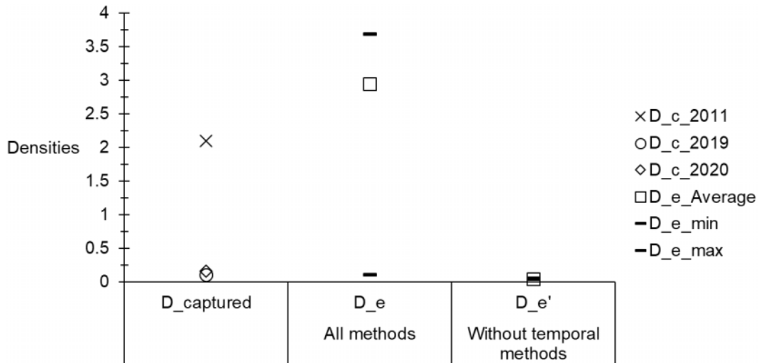
Figure 7 - Densities of captured flies ( D_c ) and corresponding effective population densities ( D_e ) while considering the whole surface of Boffa (as defined in the text) occupied by tsetse flies in the HAT focus of Boffa (Guinea), for different years and different effective population size averages: with all methods, or without temporal methods.
