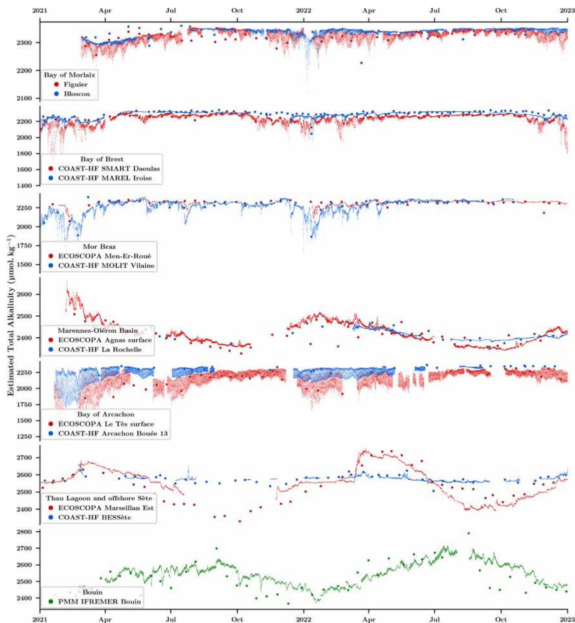
Figure 7. Estimated total alkalinity A_T time series for farming (red) and oceanic sites (blue) based on multiple regression analyses using seawater temperature, salinity, and nutrient data. The larger red and blue dots show discrete A_T values measured by the SNAPO-CO 2 laboratory. The lower plot (in green) shows the A_T evolutions inside the Bouin oyster growth facility at Ifremer.
