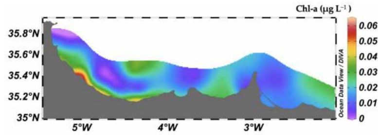
Figure 4. Distribution of surface chlorophyll-a ( \mu\text{g L}^{-1} ).
