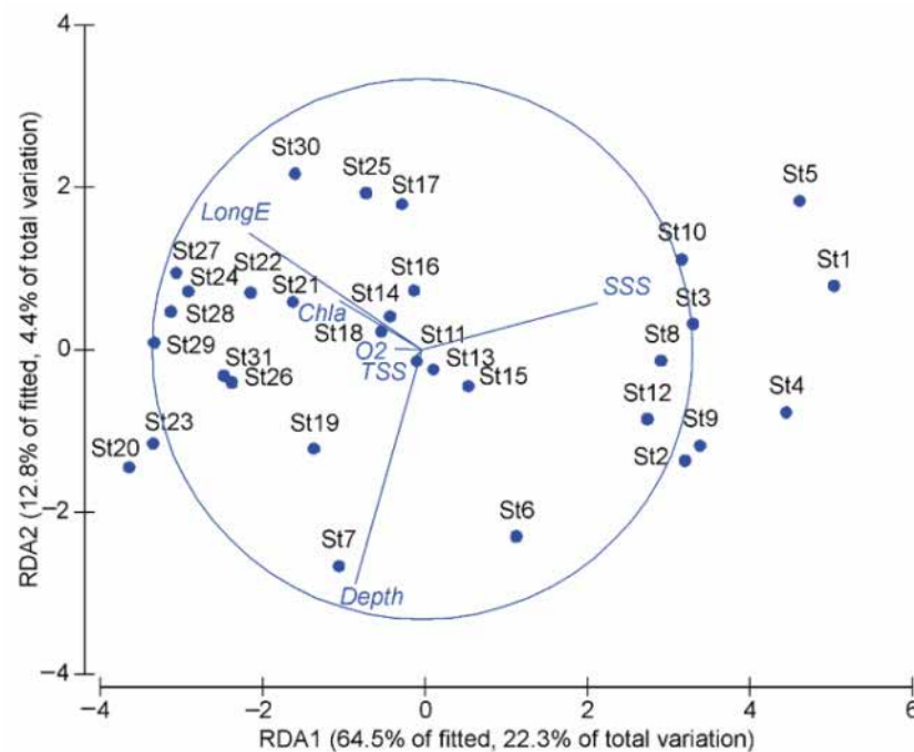
Figure 13. Result of the distance-based redundancy analysis (dbRDA) showing the effect of the spatial variation in zooplankton community structure related to the predictor variables selected through the best linear models based on distance (DistLM).
