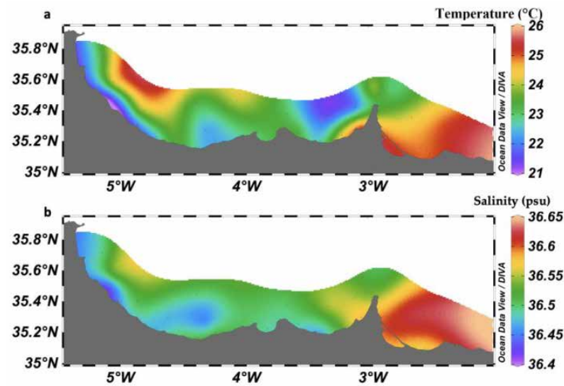
Figure 2. Distribution of the surface (a) temperature (°C) and (b) salinity (psu).
