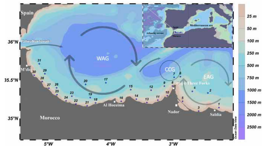
Figure 1. Sampling area and position of stations in the Moroccan Mediterranean Sea. Alboran gyres (WAG, CCG, and EAG) are represented by the gray arrows.
