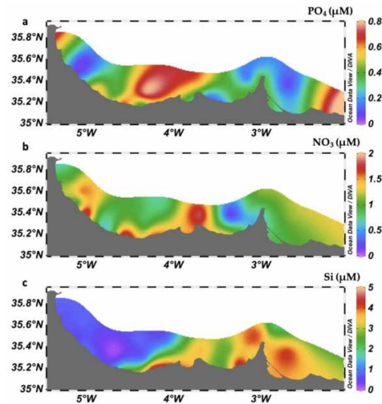
Figure 3. Distribution of surface nutrients: (a) phosphates ( \text{PO}_4 ), (b) nitrates ( \text{NO}_3 ), and (c) silicates (Si) in \mu\text{M} .
