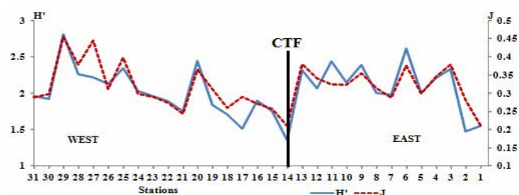
Figure 10. Spatial variation of copepod diversity indices: Shannon index (H') and Pielou index (J).
