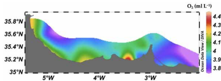
Figure 5. Distribution of surface dissolved oxygen ( \text{mL L}^{-1} ).
