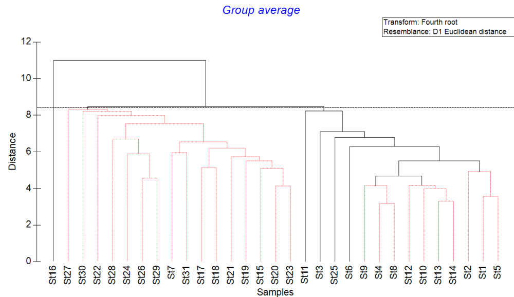
Figure 11. Dendrogram for hierarchical clustering of the zooplankton sampling stations, using group-average linking of Euclidean distance calculated on fourth root transformed abundance data.
