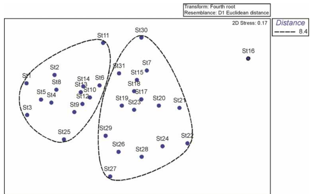
Figure 12. Non-metric multidimensional scaling (NMDS) of the spatial variation in the structure of the mesozooplankton communities in the study area.
