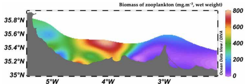
Figure 8. Spatial distribution of total mesozooplankton wet biomass ( \text{mg.m}^{-3} ) eastward.
