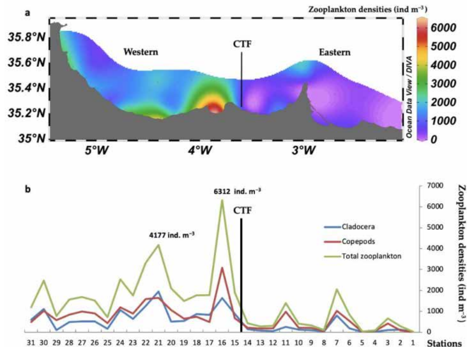
Figure 9. Spatial distribution of (a) total mesozooplankton abundance (ind.m -3 ) eastward and (b) the abundances of total mesozooplankton, copepods, and Cladocera along the study area. CTF stands for Al Hoceima.
