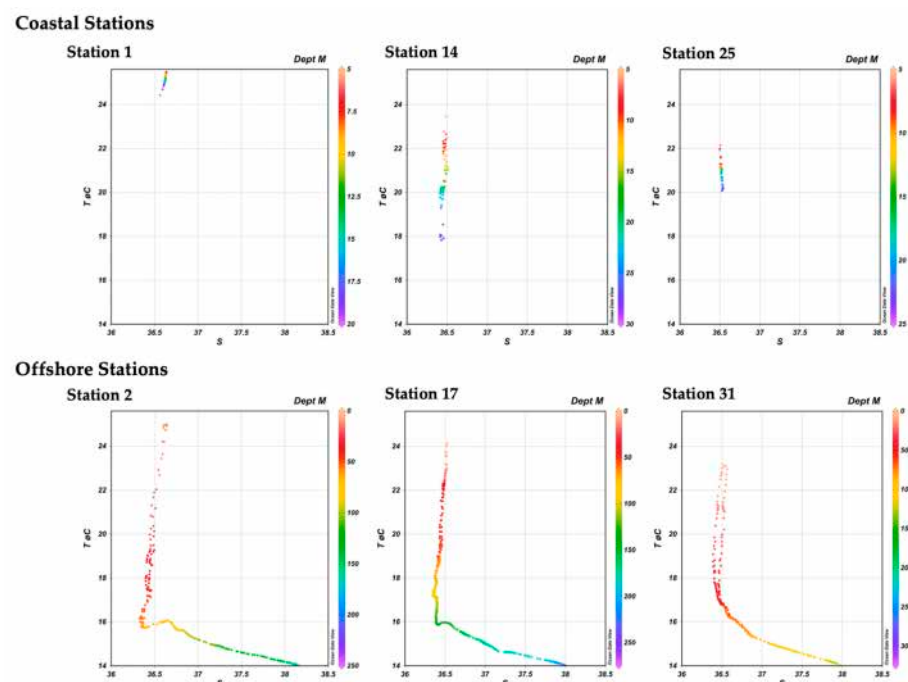
Figure 6. Vertical distribution of temperature (T in ^{\circ}\text{C} ) and salinity (psu) of representative coastal and offshore stations.
