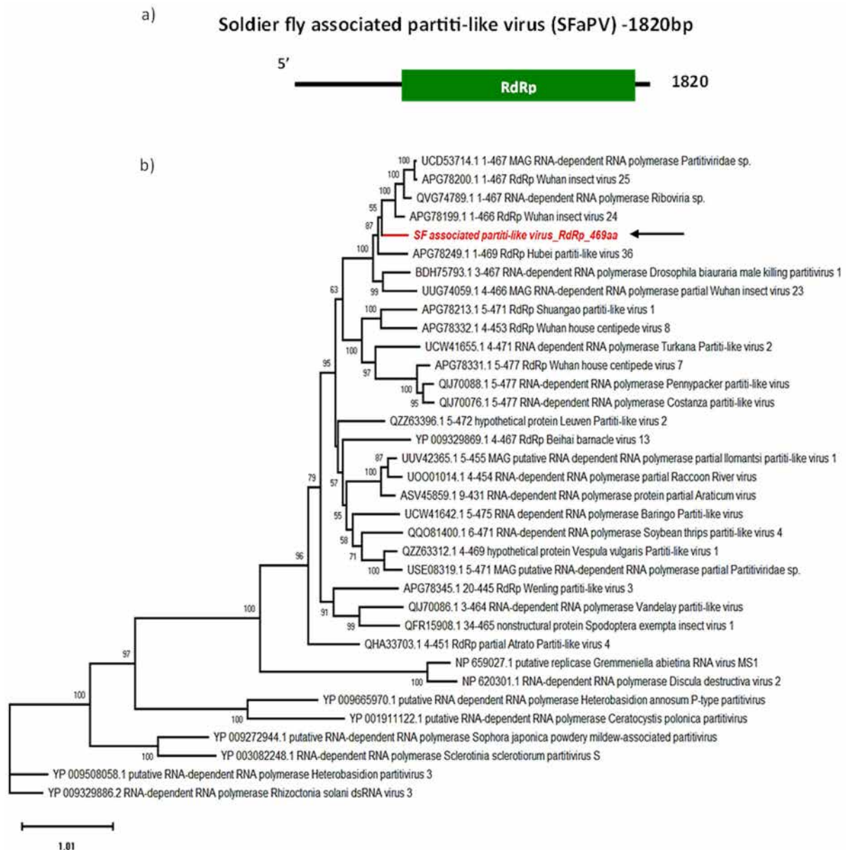
Figure 4. Genome organisation of SFaPV (a) showing single ORF encoding RdRp. For phylogenetic analysis of RdRp (b), the amino acid sequence of SFaPV (highlighted in red and indicated with arrow) is shown along with aligned reference sequences. Maximum Likelihood tree is constructed with 1000 bootstrap replicates and JTT substitution matrix with four gamma-variable sites. The scale bar refers to the number of amino acid changes per site. Bootstrap support >50% are shown at the nodes.
