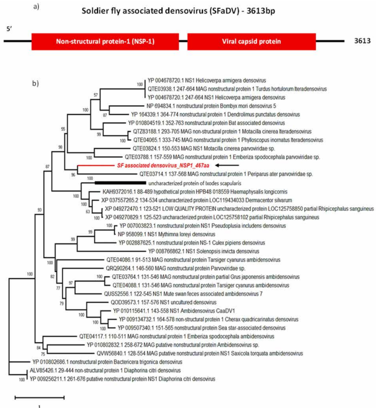
Figure 6. Genome organisation of SFaDV (a) showing two ORFs encoding NSP-1 and viral capsid protein. For phylogenetic analysis of NS1 (b), the amino acid sequence of SFaDV (highlighted in red and indicated with arrow) is shown along with aligned reference sequences. Maximum Likelihood tree is constructed with 1000 bootstrap replicates and JTT substitution matrix with four gamma-variable sites. The scale bar refers to the number of amino acid changes per site. Bootstrap support values >50% are shown at the nodes.
