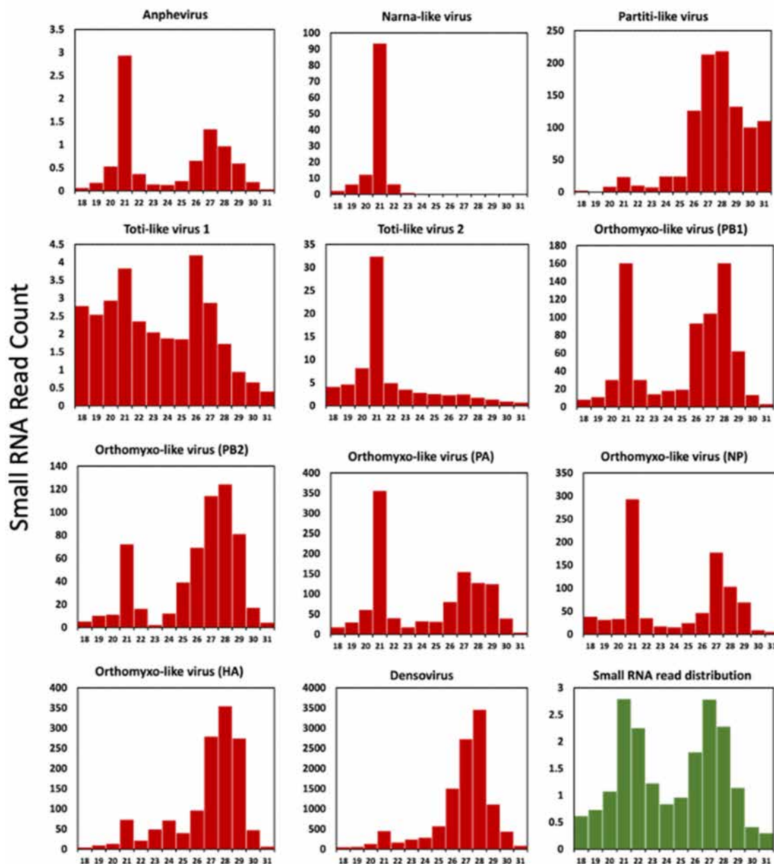
Figure 7. Virus-derived small interfering RNA profile of recently identified soldier fly-associated viruses. Read count on Y-axis is in thousands. The chart with green bars represents total small RNA read distribution, read count on Y-axis is in millions.
