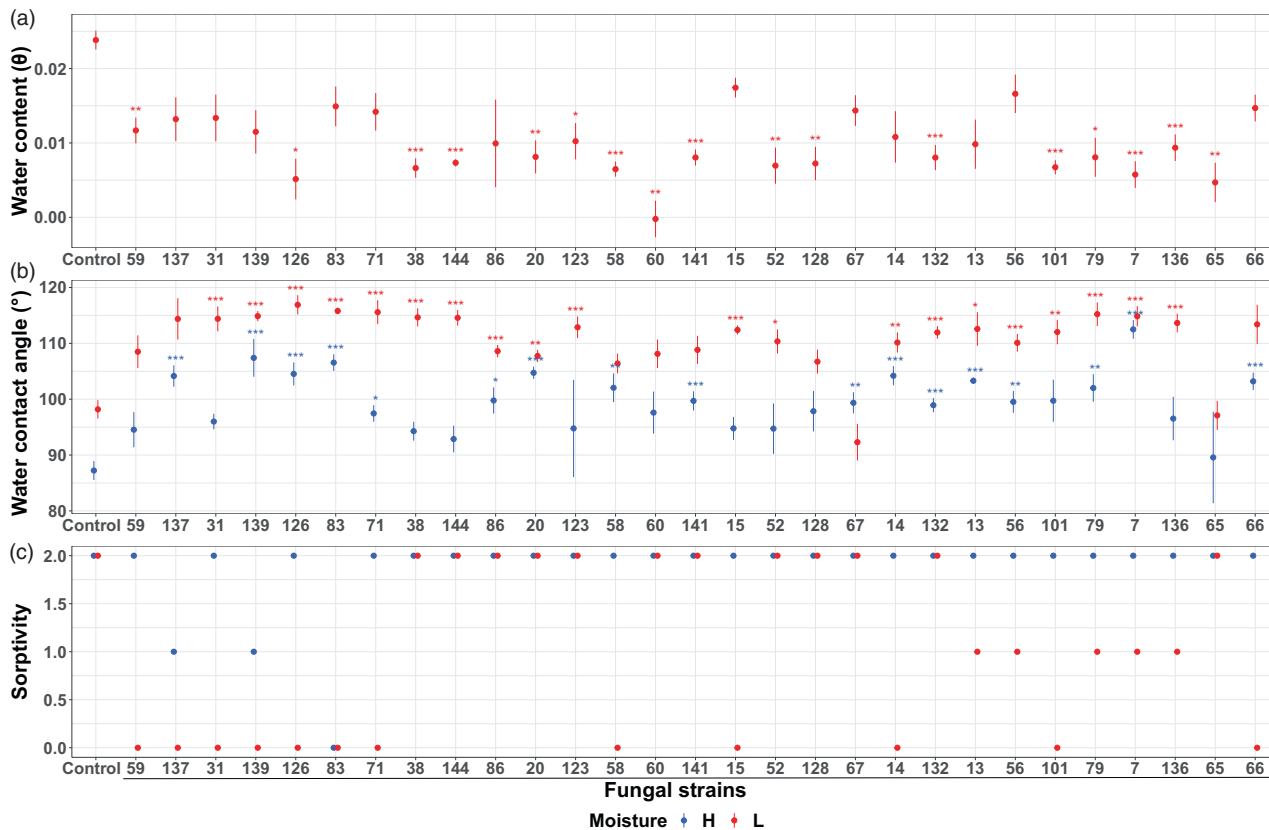
FIGURE 4 Effect of fungal inoculation on the soil hydrological properties: gravimetric water content ( \theta ) (A), soil water hydrophobicity as indicated by the soil water contact angle (WCA) (B), and sorptivity (C) after 8 weeks of incubation. Bars represent standard error. Asterisks indicate significant differences compared to the non-inoculated control: * p < 0.05 , ** p < 0.01 , and *** p < 0.001 . H and L indicate high and low soil moisture, respectively. The sequence of strains in the x-axis depicts the phylogenetic distance (Figure A, Appendix A3). The ANOVA is shown in Appendix A4, Table C. Means, standard error, p -values, and significance are shown in Appendix A4, Table F. Raw data are shown in Appendix A3, Figure G.
