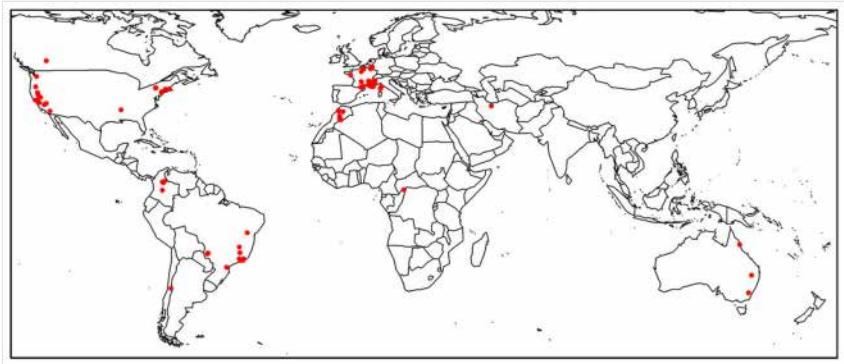
Figure 4. doi World distribution of hoverfly specimens in the collection of Jean Timon-David.
