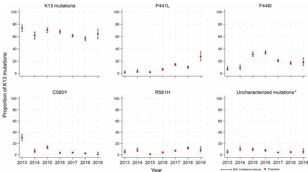
Fig. 4 Proportion of K13 mutations from 2013 to 2019. The y-axis represents K13 mutants proportion with 95% confidence intervals while the x-axis denotes the years from 2013 to 2019. # K13 mutations where the association with parasite clearance has not yet been established. The uncharacterized mutations are A621V, A626S, C469F, C469Y, C542Y, D109Y, D452E, D584V, E208K, E321K, F614L, G533A, G533D, G533S, G718S, I205T, K189T, K438N, K479I, K586E, M562I, N264I, N490H, N525Y, R265P, R528S, R529G, R575K, S423N, T192I, T535M, V193E, V494I, V534G, W611C
