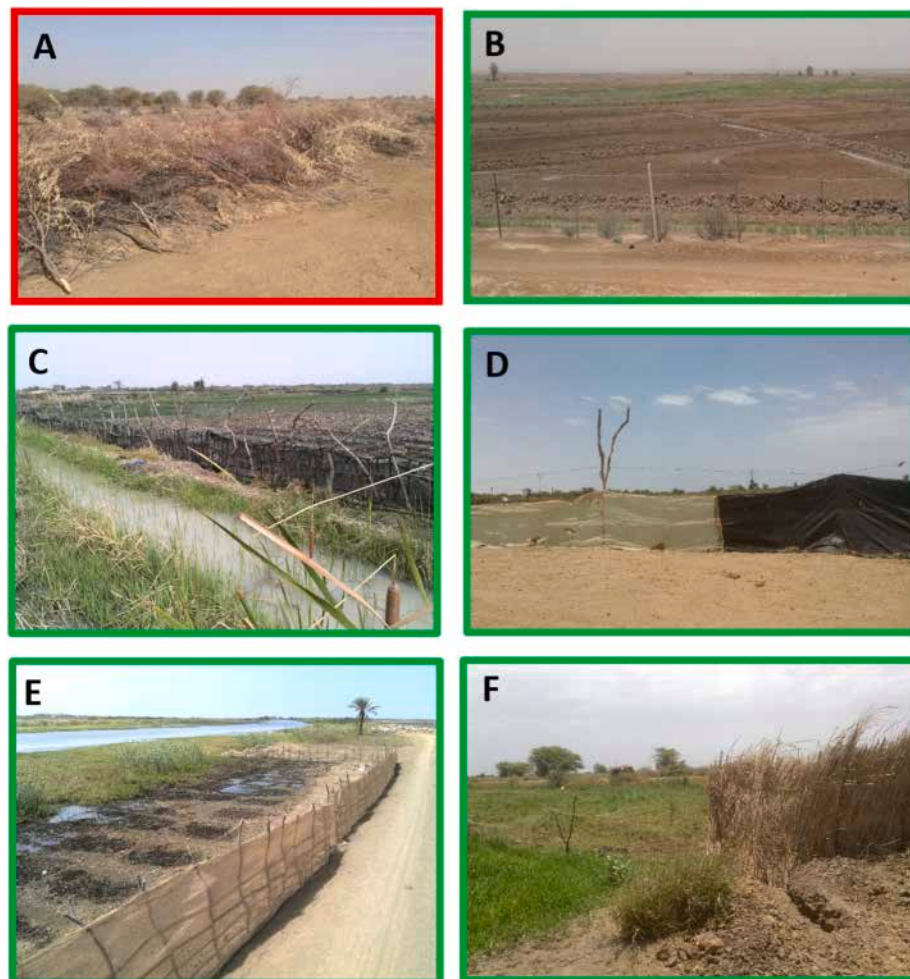
Fig. 2. Examples of rodent-favorable and unfavorable fences in cultivated plots in the River Senegal valley.
