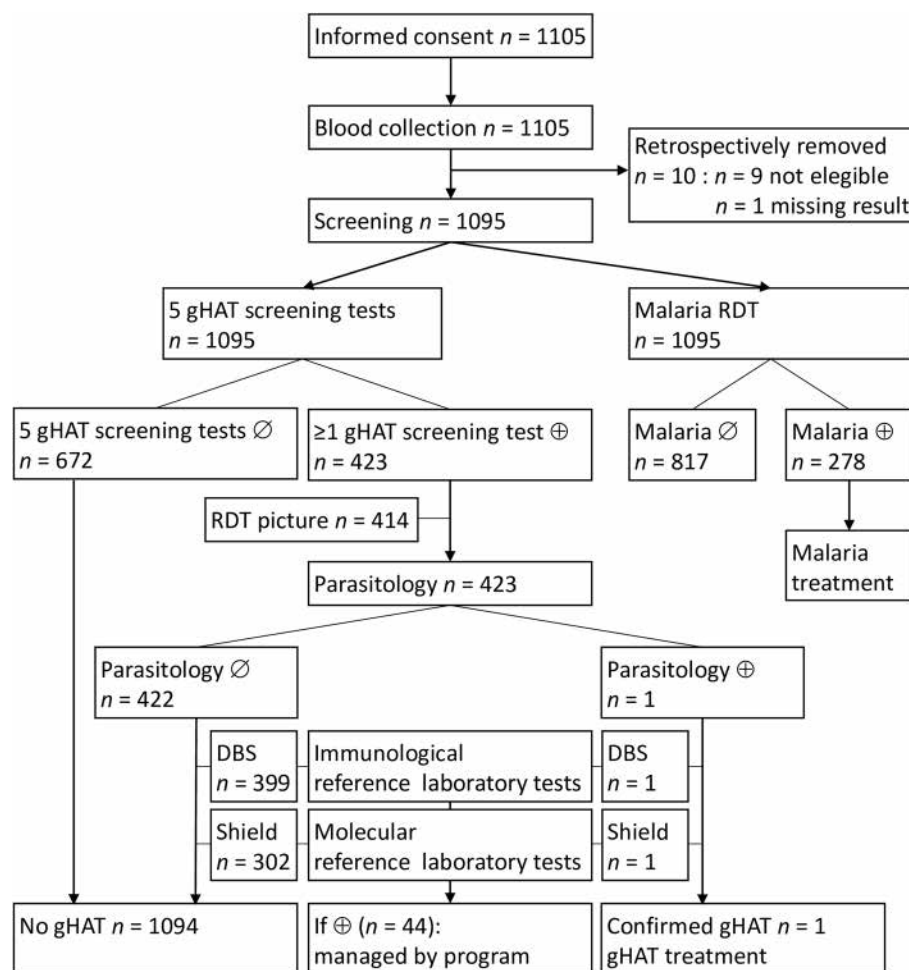
Fig. 1 Summary of the test algorithm and data interpretation. gHAT gambiense Human African trypanosomiasis; RDT rapid diagnostic test; Ø negative test result; ⊕ positive test result; DBS dried blood spot; Shield : blood in DNA/RNA shield buffer
