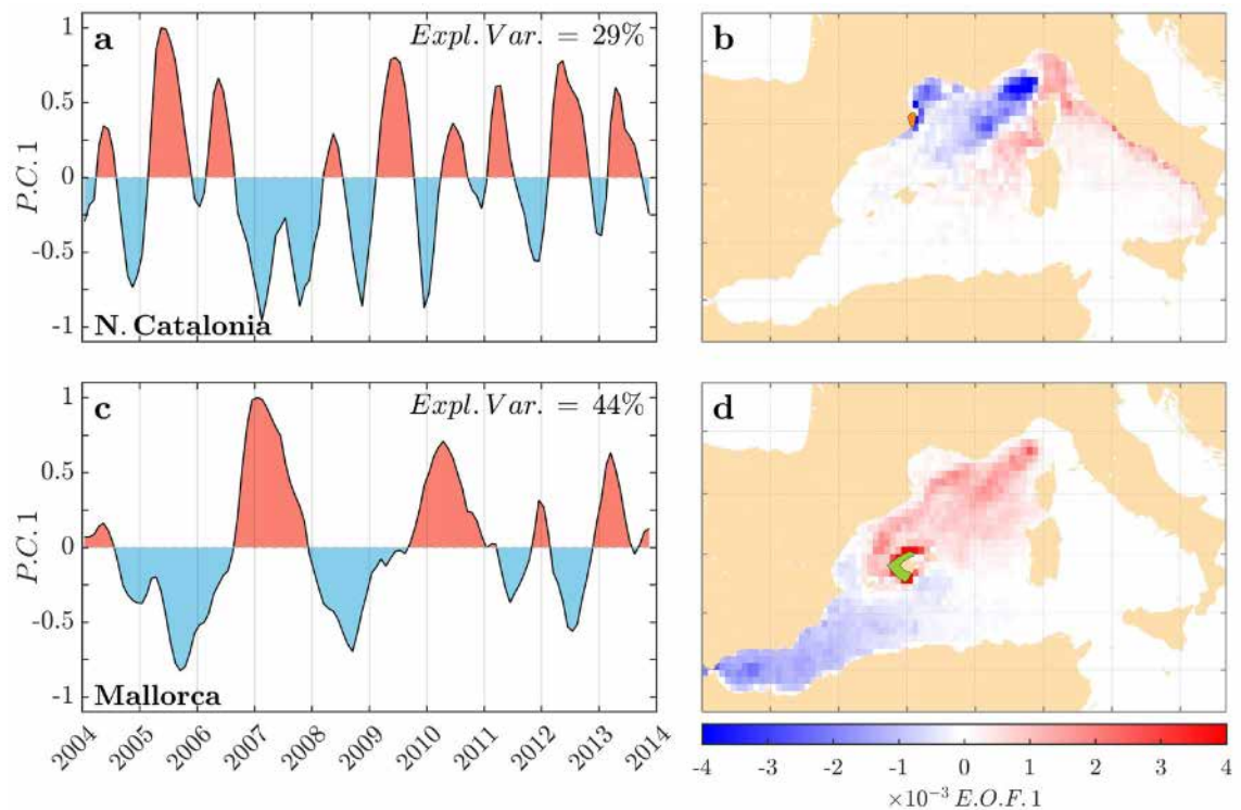
Figure 3. Prevailing sources and interannual patterns of LPDP arriving at the target areas after eight months. Temporal (a,c) and spatial (b,d) representation of the first principal component (PC1) of empirical orthogonal function (EOF) analysis conducted on source areas of individuals based on 120 monthly origin maps (2003–2014) (more details in “Methods”). The results are for N. Catalonia (a,b) and Mallorca (c,d). The total explained variance was 29% for N. Catalonia and 44% for Mallorca. Positive PC and EOF values are in red, and negative values are in blue. Original source maps can be reconstructed using the climatology (Fig. 1b,c) and adding the product of PC1 by EOF values. Therefore, intensified influence as source areas emerges when blue/red areas (from EOF value) and PC value match (blue/red). The figure and superimposed maps were created using “M Map: A mapping package for MATLAB”, v.1.4m ( www.eoas.ubc.ca/~rich/map.html ) in MATLAB v.R2010b ( www.mathworks.com ).
