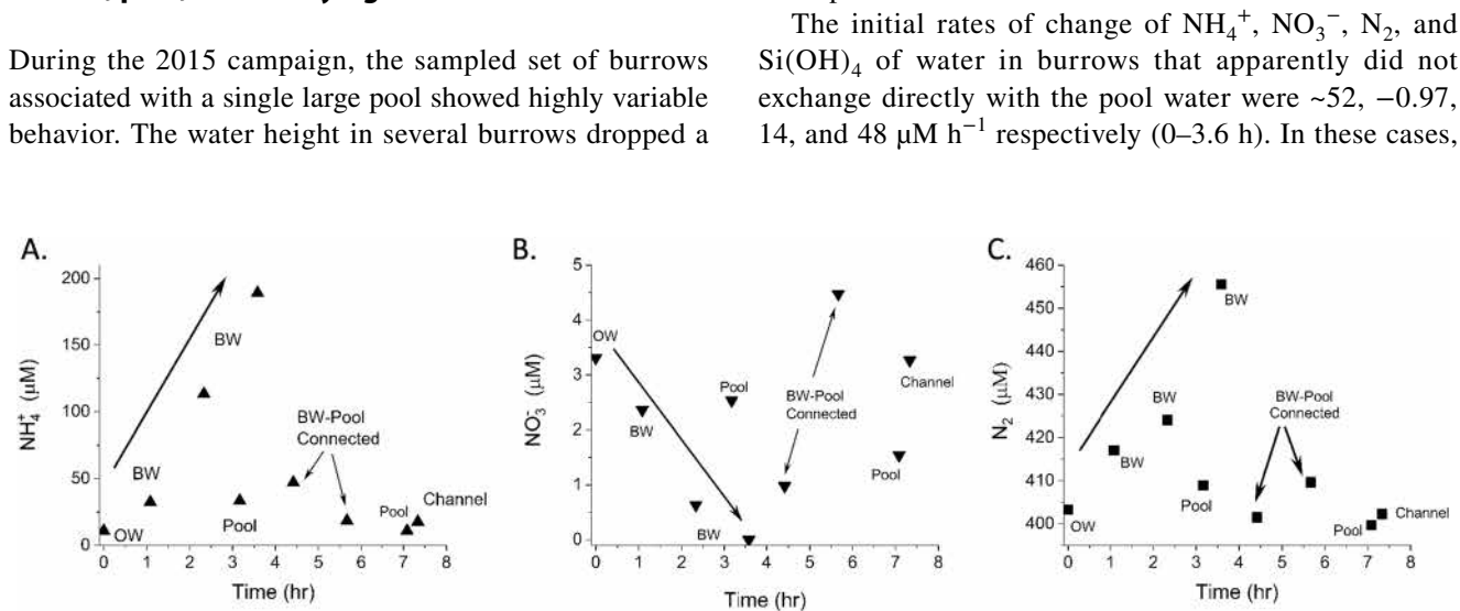
Fig. 4 Time series burrow waters, associated pool water, ebb overlying water, and channel flood water concentrations of \text{NH}_4^+ , \text{NO}_3^- , and \text{N}_2 at a single pool site during 2015 sampling. Initial time series burrow water (to ~3.6 h) reflects separate individual burrows. If the
