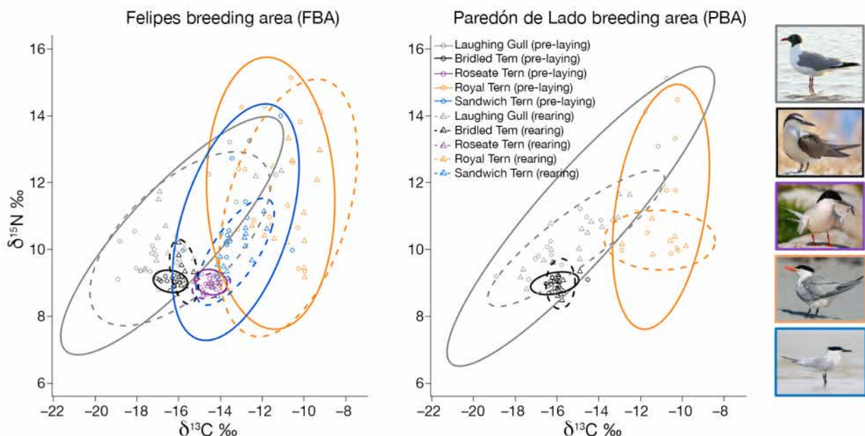
Fig. 3. Bayesian standard ellipses for corrected sample sizes representing the isotopic niches ( \delta^{13}\text{C} and \delta^{15}\text{N} ) of 5 Laridae species from 2 breeding areas in central-northern Cuba during 2 phases (pre-laying and rearing) of the 2021 breeding season
