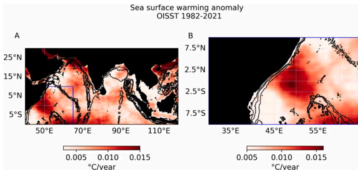
Fig. 3. The WIO is a global warming hotspot within the Indian Ocean basin. The maps represent the anomaly of sea surface warming (relative to the annual mean trend over the Indian Ocean) at A ) the WIO basin level and B ) along the East African coast using linear regression on the National Oceanic and Atmospheric Administration \frac{1}{4}^\circ Daily Optimum Interpolation Sea Surface Temperature between 1982 and 2021.
