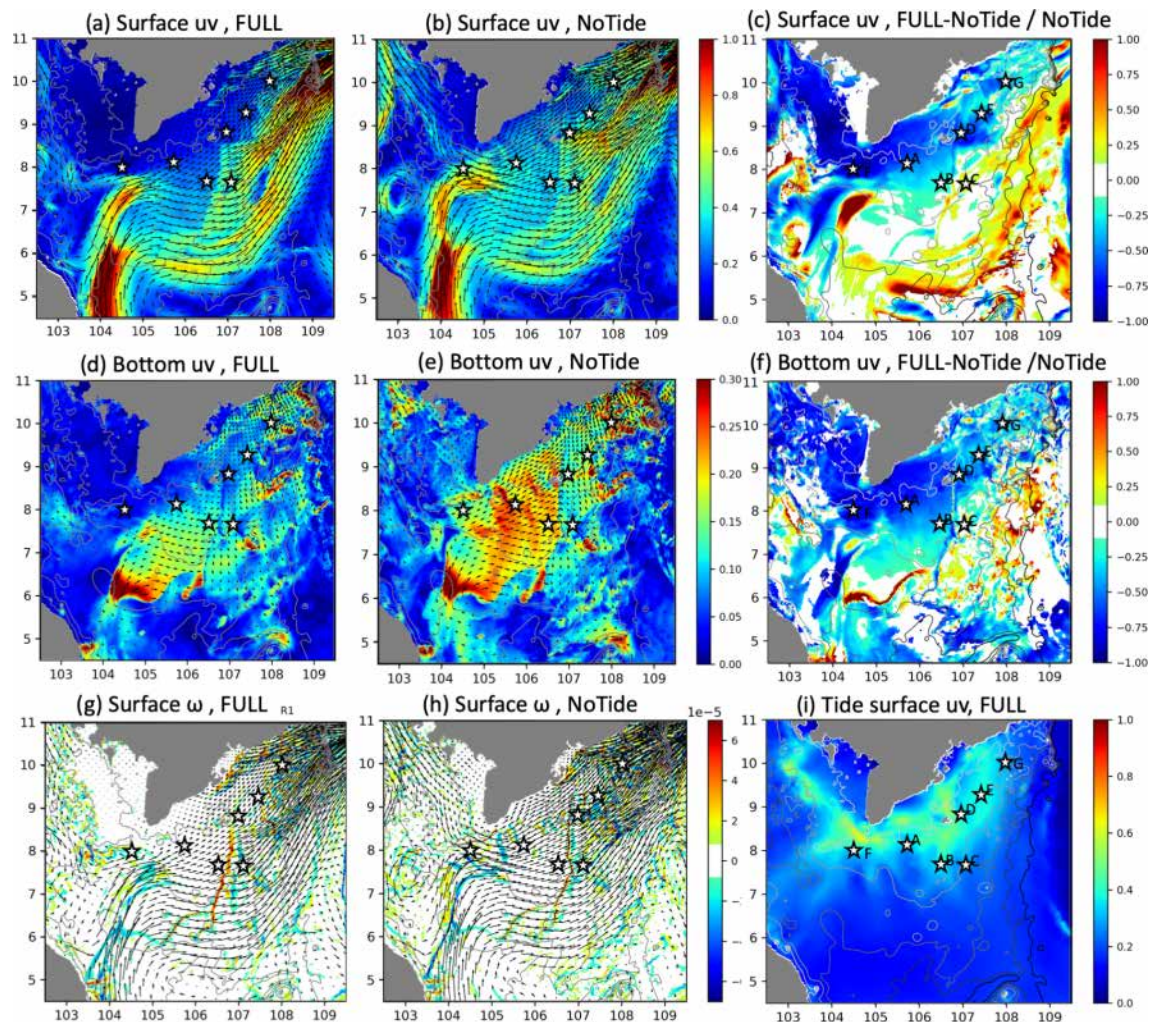
Figure 5. Surface (a, b) and bottom (d, e) horizontal velocity on 16 July 2018 in M17 from the FULL (a, d) and NoTide (b, e) ensembles (in \text{m s}^{-1} : colours indicate the speed and arrows the direction). (c, f) Relative differences between FULL and NoTide [no unit]. (g, h) Surface vertical velocity in FULL (g) and NoTide (h) (in \text{m s}^{-1} : arrows show the surface horizontal velocity). (i) Surface tidal speed in FULL [ \text{m s}^{-1} ].
