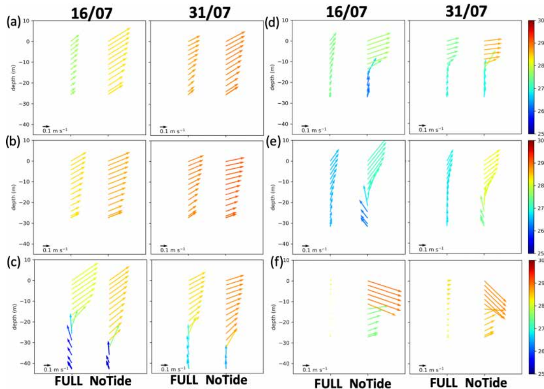
Figure 6. Profiles of temperature (colour; in ^{\circ}\text{C} ) and horizontal velocity (arrows; in \text{m s}^{-1} ) on 16 July and 31 July 2018 at points A, B, C, D, E, and F shown in Figs. 4, 5, and 8 in M17 for the FULL and NoTide ensembles.
