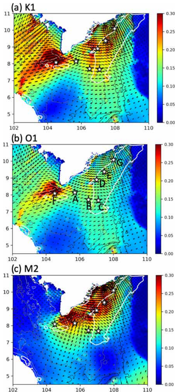
Figure 8. Depth-averaged tidal current ellipses and current intensity [ \text{ms}^{-1} ] in M17 from the FULL ensemble for the three significant tidal components in the MKU region: K1, O1, and M2. The white lines show the 0.2^\circ\text{C} isoline of the difference between JJAS-averaged SST in FULL and in NoTide, corresponding to the area where upwelling is much stronger in FULL than in NoTide in Fig. 1.
