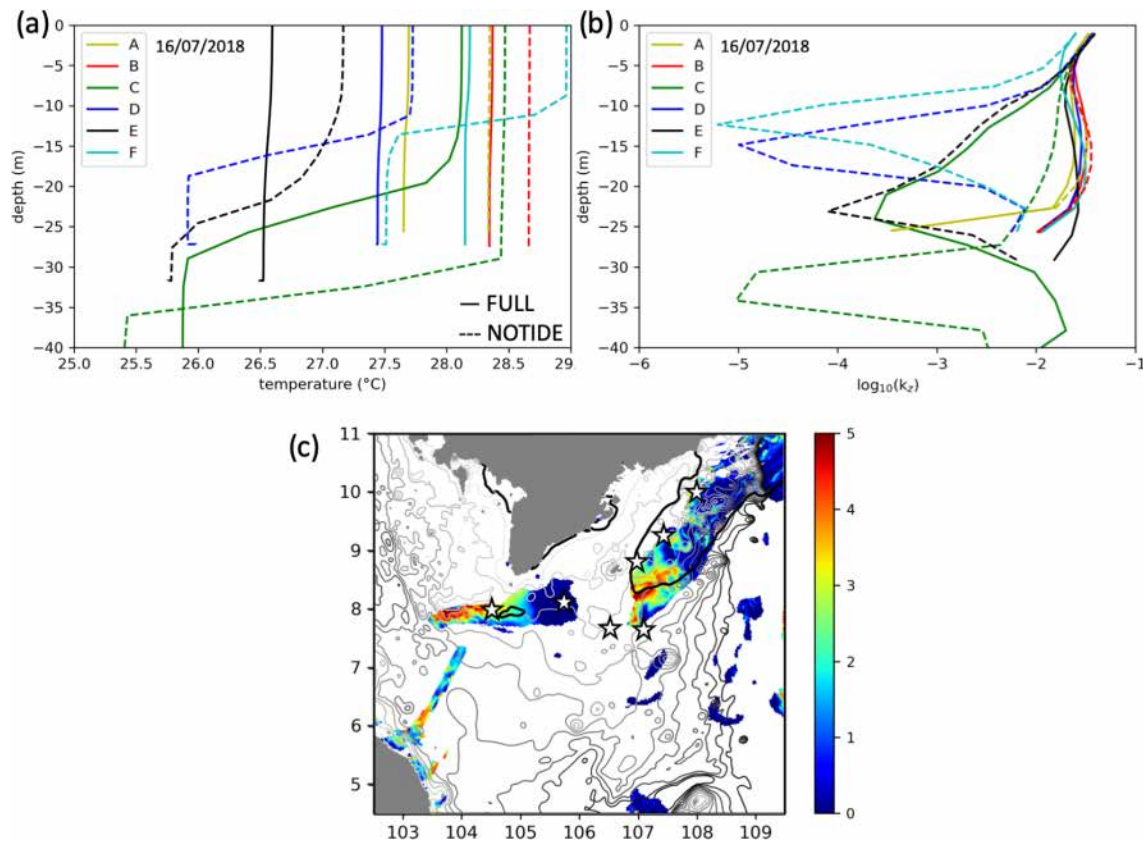
Figure 9. Profiles of temperature (a; in ^\circ\text{C} ) and diffusivity coefficient k_z (b; in \text{m}^2\text{s}^{-1} , logarithmic scale) on 16 July 2018 at points A, B, C, D, E, and F shown in Figs. 4, 5, and 8 in M17 from the FULL (solid lines) and NoTide (dashed line) ensembles. (c) Map of the maximum over the water column of the difference in diffusivity coefficient between FULL and NoTide, \Delta\log_{10}(k_z) , from the same day as (b), plotted for areas where the FULL – NoTide SST difference exceeds 0.4^\circ\text{C} . The black line shows the T_o = 27.6^\circ\text{C} surface isotherm.
