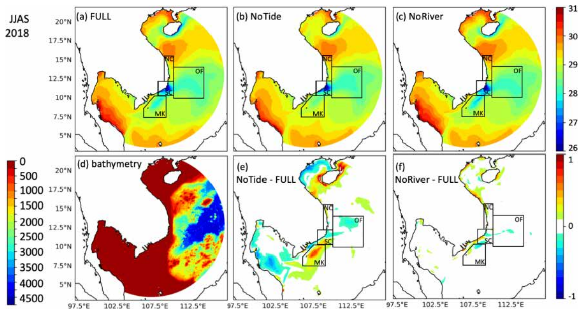
Figure 1. Ensemble average summer SST in June–September 2018 from the FULL (a), NoTide (b), and NoRiver (c) ensembles and the difference between the NoTide and FULL (e) and the NoRiver and FULL (f) ensembles [ ^{\circ}\text{C} ]. (d) Bathymetry of the domain [m]. Colour bars for panels (a)–(c) and (e)–(f) are provided at the top and bottom right, and the colour bar for panel (d) is at the bottom left. Upwelling areas have the following names and coordinates: boxNC (12.2–15.5° N, 108.7–109.9° E), boxSC (10.3–12.2° N, 108–109.9° E), boxOF (10–14° N, 109.9–114° E), and boxMK (at depth > 17 m; 7.5–10.3° N, 106–109° E).
