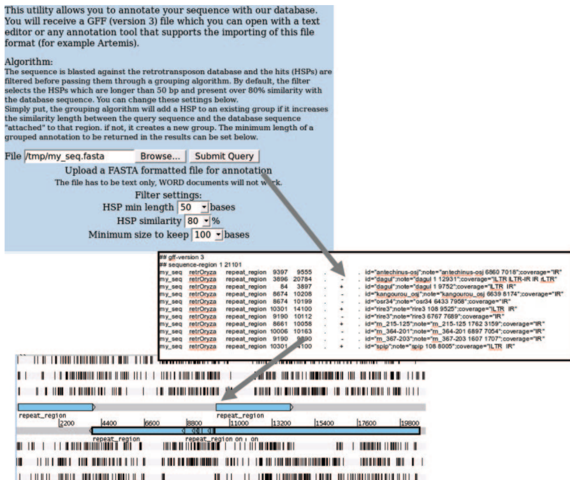
Figure 3. The annotation process consists of uploading a FASTA formatted file to the server which will return a file to the user after the analysis. This file is in the GFF format which can be opened with a text editor or loaded into an annotation editor such as Artemis.
