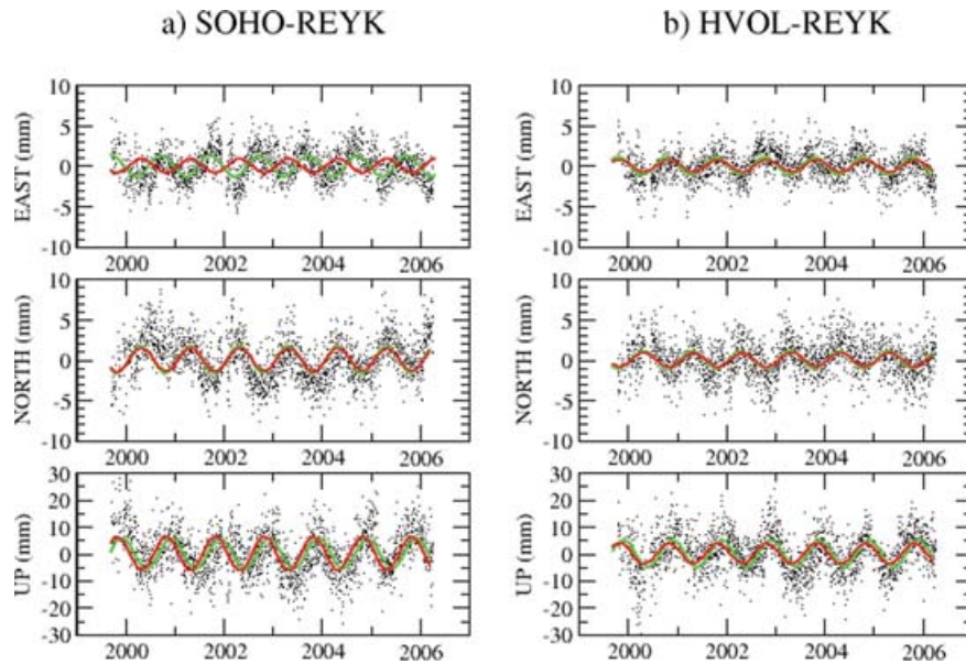
Figure 9. Time-series of east, north and vertical component of the SOHO and HVOL GPS stations (reference station is REYK). The linear trend (for SOHO, respectively 16.63 mm \text{yr}^{-1} , -8.08 mm \text{yr}^{-1} and 10.11 mm \text{yr}^{-1} for the east, north and vertical component; for HVOL, respectively 18.98 mm \text{yr}^{-1} , -6.94 mm \text{yr}^{-1} and 8.51 mm \text{yr}^{-1} for the east, north and vertical component) has been removed. The green curve is a fit of data by a function A \cos(wt + \phi) (for SOHO, the phase \phi is respectively 1.73, -2 and 0.42 for east, north and vertical component; for HVOL \phi is, respectively, 1.30, -1.94 and 0.57 for east, north and vertical component). The red curve is for the elastic model (see Fig. 11) considering a maximum of ice thickness at the beginning of May.
