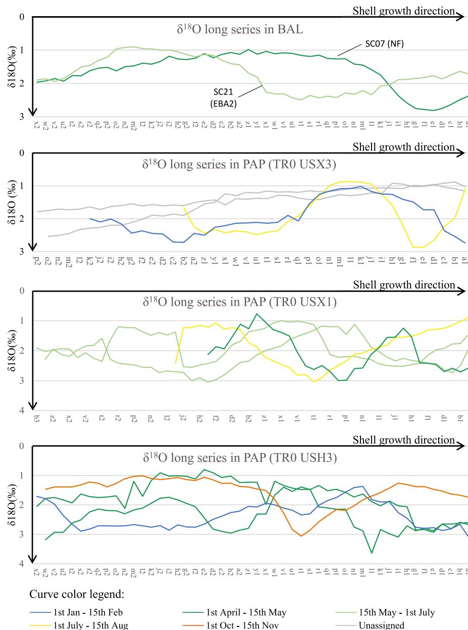
Fig. 4. Long series of \delta^{18}\text{O} (‰) measured along limpet shell from the apex to the margin. Letters on abscissas represent sampling positions within the shell axis with “a1” (on the right of abscissa) being the sample the closest from the margin. Each plot represents one stratigraphy unit. Ordinate axes are reversed so temperature direction follows graphical \delta^{18}\text{O} direction. Curve colors indicate season assignment: greens (spring), yellow and orange (summer), brown (autumn), blue (winter) and grey (no assignment).
