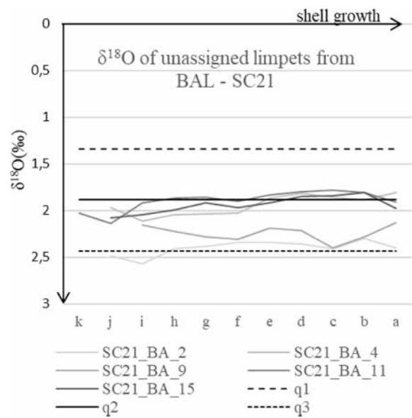
Fig. D. Examples of \delta^{18}\text{O} (‰) profiles from limpet shells with no fished season assignment: \delta^{18}\text{O} measured along limpet shell margins within the SC21 stratigraphic unit of Beg ar Loued site. Letters from “k” to “a” on the abscissa represent sampling positions within the shell margin with “a” being the sampling point the closest from the margin. Ordinate axes are reversed so temperature direction follows graphical \delta^{18}\text{O} direction.
