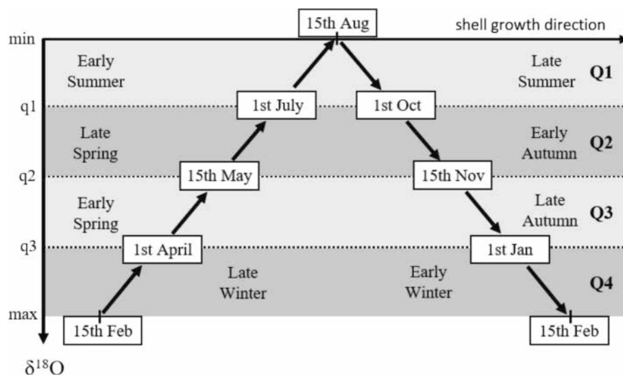
Fig. 3. Schematic representation of the annual temperature cycle recorded as a shell \delta^{18}\text{O} profile. The harvesting season is determined by the marginal \delta^{18}\text{O} values coupled with the last few samples trend.
