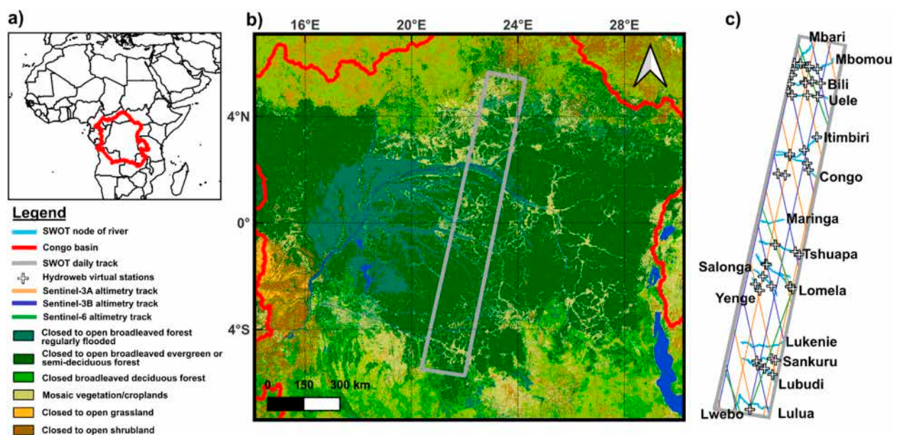
FIGURE 1 Location of the study site. (A) Location of the Congo Basin, (B) land cover over the Cuvette Centrale and (C) SWOT daily node track acquired on April 2023 over the Cuvette Centrale (rectangular gray frame).
