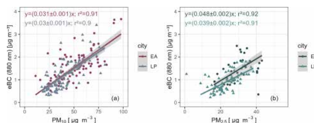
Figure 4. Scatterplot of daily averaged eBC mass concentrations vs. PM 10 (a) and PM 2.5 (b) concentrations at both sites (two outliers were excluded from the ordinary least-squares regression displayed in the right panel).
