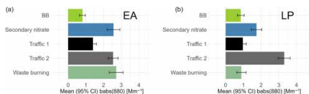
Figure 9. Mean contribution to absorption at a wavelength of 880 nm of the five sources of PM 10 resolved by Mardoñez et al. (2023) (a: EA, b: LP), who presented a positive contribution to total absorption and a p value < 0.05 in the multilinear ordinary least-squares regression.
