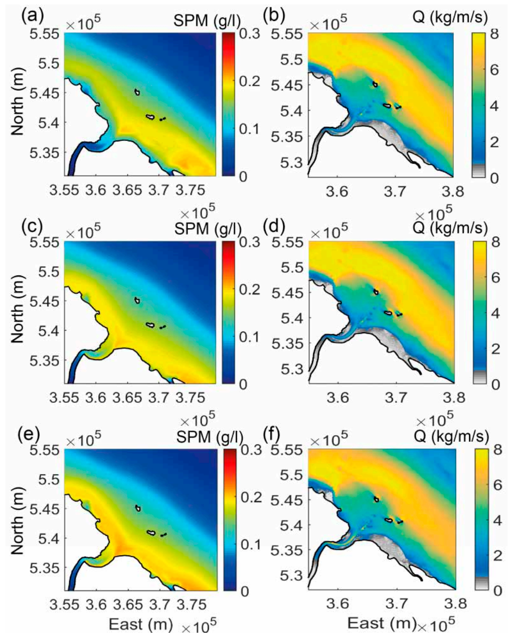
Figure 7. SPM and sediment transport outputs for different conditions during the dry season. (a) SPM and (b) transport with tides and wind-generated currents, (c) SPM and (d) transport, including wave currents, (e) SPM and (f) transport using the Ng formulation for the wave–mud interaction.
