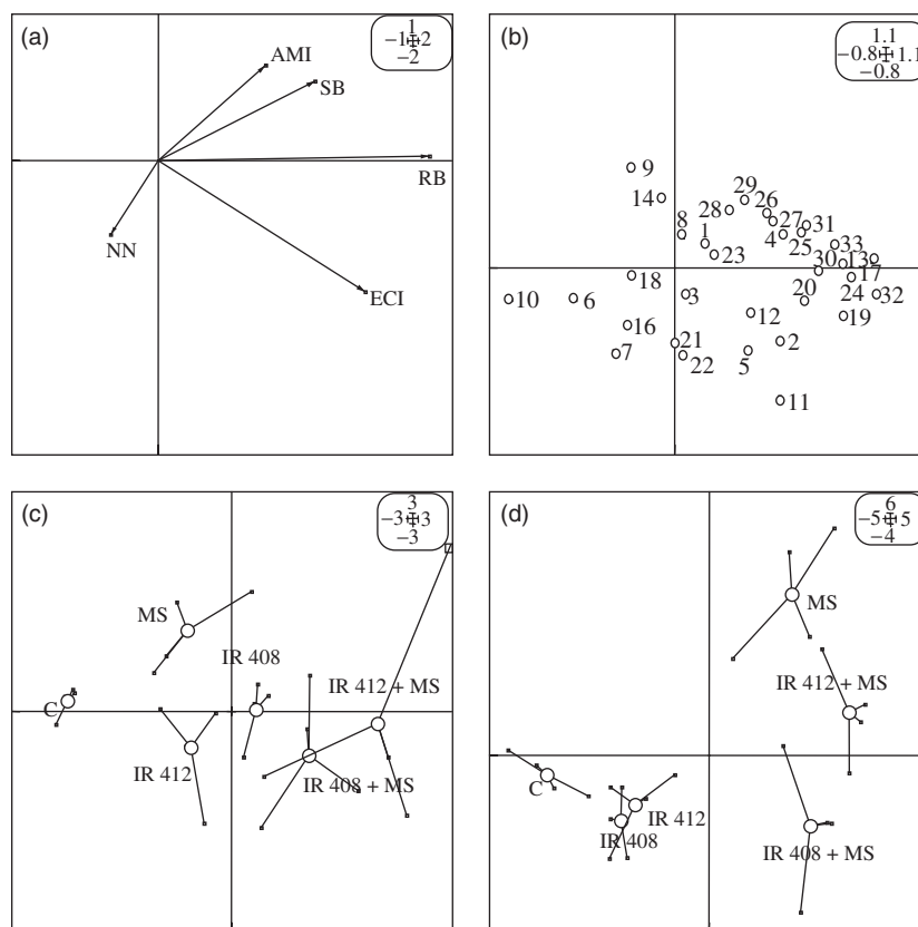
Fig. 4. Co-inertia analysis of substrate-induced respiration (SIR) responses of soils inoculated or not with Sclerotinia dictyosporum isolates IR408 and IR412 and amended or not with mound powder. In the four panels (a–d), the top-right inset gives the minimum and maximum of the horizontal and vertical coordinates. (a) Factor map of plant growth. Mycorrhizal and rhizobial variables: SB, shoot biomass; RB, root biomass; AMI, arbuscular mycorrhizal colonization index; ECI, ectomycorrhizal colonization index; NN, number of nodules per plant. (b) Factor map of SIR responses. 1, L-glutamine; 2, L-arginine; 3, L-serine; 4, L-histidine; 5, phenylalanine; 6, L-asparagine; 7, L-tyrosine; 8, L-glutamic acid; 9, L-lysine; 10, L-cysteine; 11, D-glucose; 12, D-mannose; 13, sucrose; 14, D-glucosamine; 15, N-methyl-D-glucamine; 16, succinamide; 17, 2-keto-glutaric acid; 18, 3-hydroxy-butyric acid; 19, ascorbic acid; 20, D-quinic acid; 21, D,L-malic acid; 22, formic acid; 23, fumaric acid; 24, gallic acid; 25, gluconic acid; 26, keto-butyric acid; 27, malonic acid; 28, oxalic acid; 29, succinic acid; 30, tartaric acid; 31, trisodium citrate; 32, uric acid; 33, cyclohexane. (c) Factor map of plant growth. Microbial and soil sample variables: C, control; MS, soil amended with Macrotermes subhyalinus mound powder; IR408, soil inoculated with S. dictyosporum strain IR408; IR412, soil inoculated with S. dictyosporum strain IR412; IR408+MS, soil inoculated with S. dictyosporum strain IR408 and amended with M. subhyalinus mound powder; IR412+MS, soil inoculated with S. dictyosporum strain IR412 and amended with M. subhyalinus mound powder. The star-like diagrams represent the four replicates of each treatment, and the dot inside each star is the mean of these replicates. (d) Factor map of SIR responses of soil samples (for details, see c).
