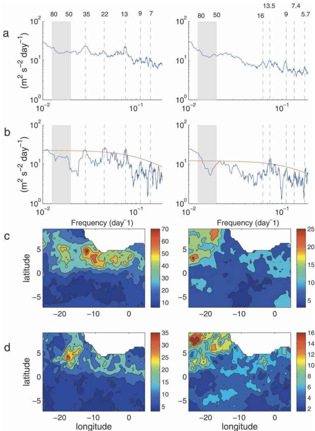
FIG. 5. (a) Mean velocity wind spectra of the (left) zonal and (right) meridional components from QuikSCAT. The mean is computed with the 2108 spectra corresponding to the grid points between 7.25°S and 9.25°N and between 25.75° and 0.25°W. The vertical lines from left to right indicate the periods of 35, 22, 13, 9, and 7 days (zonal component) and 16, 13.5, 9, 7.4, and 5.7 days (meridional component). Shadowed region indicates the 50–80-day band. (b) Same as (a) but for a point located at 0.25°N, 10.25°W. The red curve indicates the 95% confidence interval. (c), (d) Amplitude of the spectrum (left) for 13 and 7 days for the zonal component and (right) for 13.5 and 7.4 days for the meridional component.
