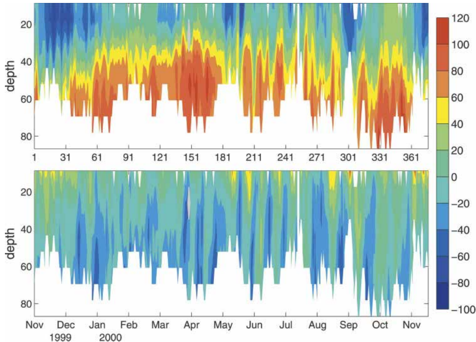
FIG. 2. (top) Zonal and (bottom) meridional velocity components ( \text{cm s}^{-1} ) from the ADCP in mooring A. Time axis is in days (top) and in months (bottom), beginning on 12 Nov 1999 and ending 24 Nov 2000.
