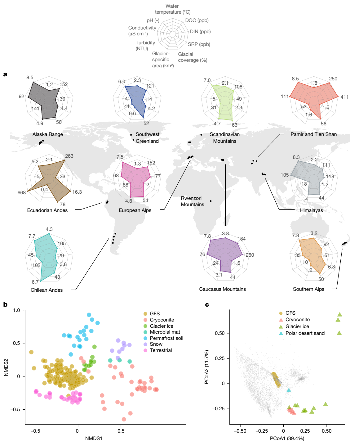
Fig. 1 | GFSs sampled by the Vanishing Glaciers project, their environmental characteristics and microbiome structure and function. a , World map showing the mountain ranges and locations (black dots) where the Vanishing Glaciers project sampled GFSs. Radar charts depict key physicochemical parameters of GFS water and glacier metrics. Shown are median values of normalized parameters. No radar chart is shown for the Rwenzori Mountains, because only one GFS was sampled. DIN, dissolved inorganic nitrogen; DOC, dissolved organic carbon; NTU, nephelometric turbidity units; ppb, parts per billion; SRP, soluble reactive phosphorus. b , Non-metric multidimensional scaling (NMDS) based on Bray–Curtis dissimilarity, illustrating the composition of bacterial communities of 152 GFSs and other cryospheric ecosystems 21 ( n_{\text{sample}} = 268 , k = 2 , stress = 0.17). Taxonomic composition of the GFS microbiome differs significantly from that of other microbiomes, as shown by both permutational analysis of variance (PERMANOVA, F_{6,264} = 8.6 , R^2 = 0.16 , P = 0.001 ;
