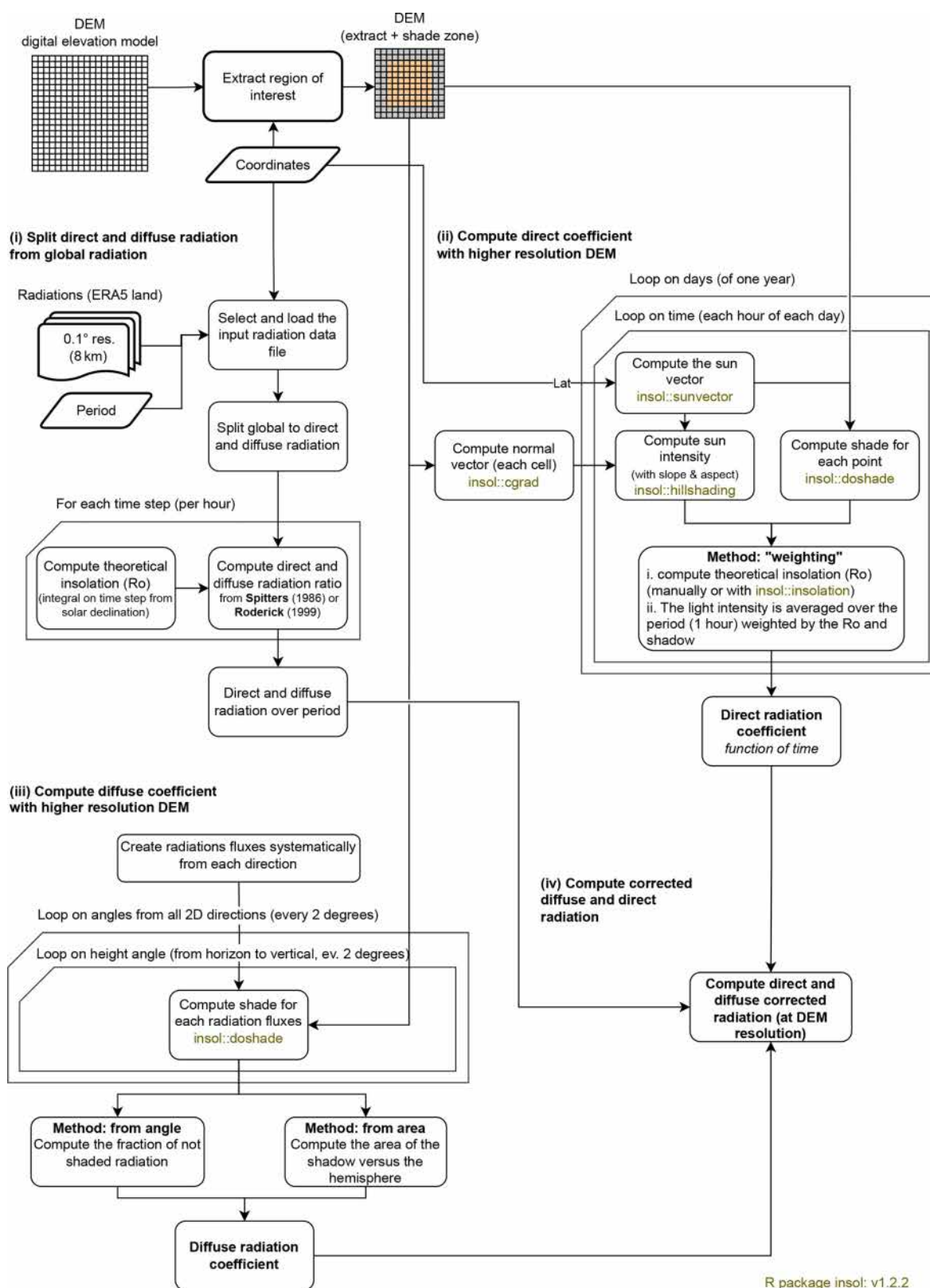
Figure 1. Simplified workflow of radiation downscaling, showing the four different steps of the procedure. The bold boxes in the top left show the input data required (DEM, coordinates, period and large-scale radiation), the green boxes show the functions of the external R package used ( insol ), the truncated boxes show the loops and the rounded boxes show the various stages.
