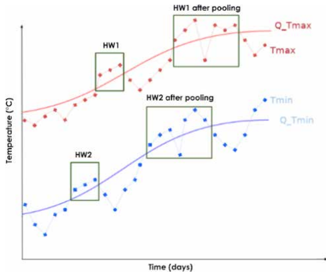
Figure 2. Detection process of heat wave: HW1 and HW2 represent events associated respectively to maximum and minimum temperature. The red and blue lines with circles are respectively maximum and minimum daily temperatures. Solid red and blue lines are respectively maximum and minimum thresholds. The x and y axes represent the time in days and the temperature in degrees Celsius. The term “after pooling” refers to the pooling of two (or more) events separated by a day characterized by the value of a given indicator below the daily XX th percentile. This figure is a “theoretical/schematic” illustration of the different types of heat waves investigated in this work.
