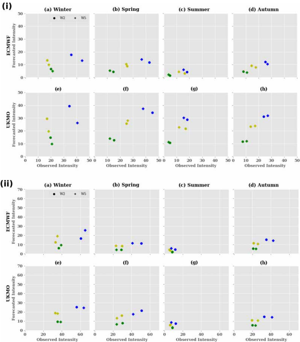
Figure 12. Evaluation of the intensity of heat waves in the forecast models and ERA5 over the period 2001–2020 during the seasons (a, e) winter, (b, f) spring, (c, g) summer and (d, h) autumn using T2m_min (i) and T2m_max (ii). The intensity of heat waves is computed independently for each initialization date within a month, and all initializations are averaged to obtain the average intensity of heat waves for the given month. Yellow, green and blue colours represent the values of intensity in the AT, GU and CO regions respectively. The dot and cross symbols represent the intensity of heat waves during week 2 (W2) and week 5 (W5) respectively. The y and x axes represent the forecasted and observed intensities in ERA5 reanalysis respectively.
