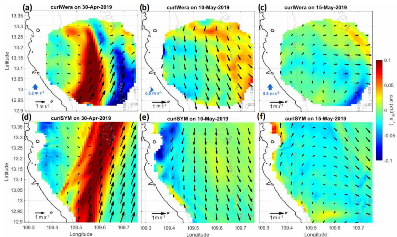
Figure 6. SSC vectors obtained from HFR (a–c) and SYMPHONIE (EASTSEA run) (d–f) of the superimposing curl of the SSC field. Blue arrows in the southwest corner denote averaged wind directions and magnitudes over the HFR domain. Isobaths are given as solid gray lines, and coastlines are represented as solid black lines.
