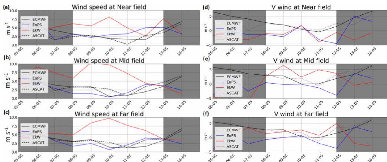
Figure 10. Columns: wind speed time series from different wind data (a, b, c) and time series of the v component of wind from wind data (d, e, f). Rows: three subdomains – near field, mid-field and far field.
