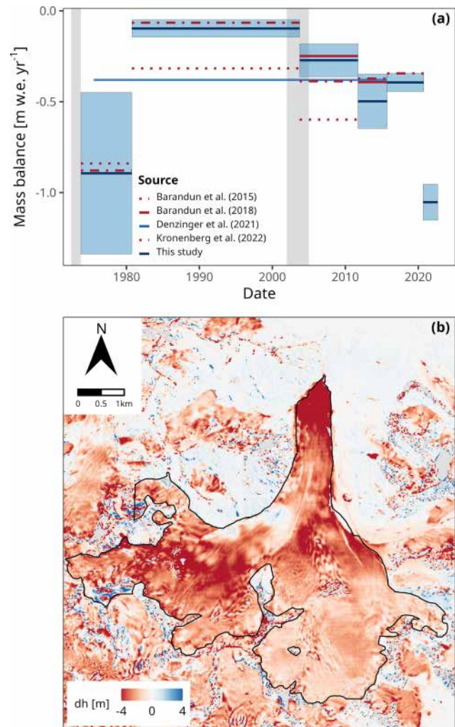
Figure 6. (a) Specific annual mass balance of Abramov glacier from our DEM differences and from previous studies; for readability, uncertainty is shown only for our results. Gray shading indicates the period of the two pulsations. (b) Pléiades DEM difference between 8 September 2020 and 5 September 2022.
