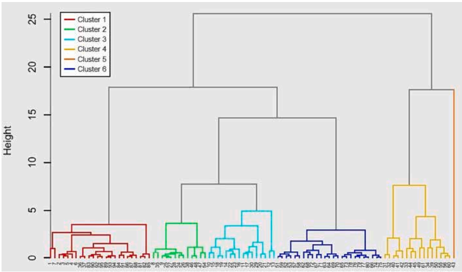
Fig. 9. Dendrogram of water quality data with hierarchical cluster analysis based on the PCA and the Ward linkage algorithm. Each cluster is defined by color.
