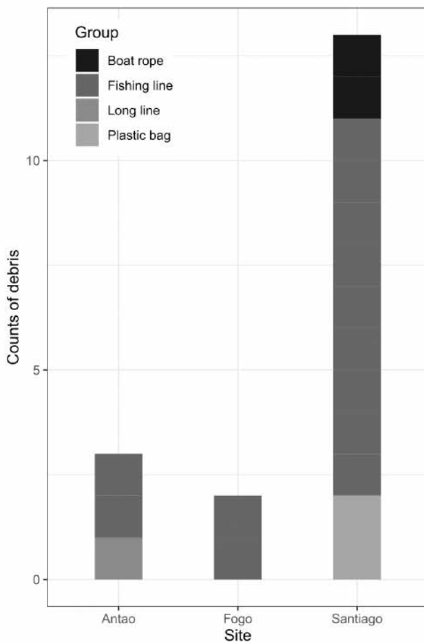
Fig. 4. Count of debris observed at the surveyed islands revealed significant differences between Santiago and the other islands (Tukey HSD test: Santiago–Fogo p_{adj} = 0.001 ; Santiago–Antão p_{adj} = 0.002 ; Fogo–Antão p_{adj} = 0.925 )
