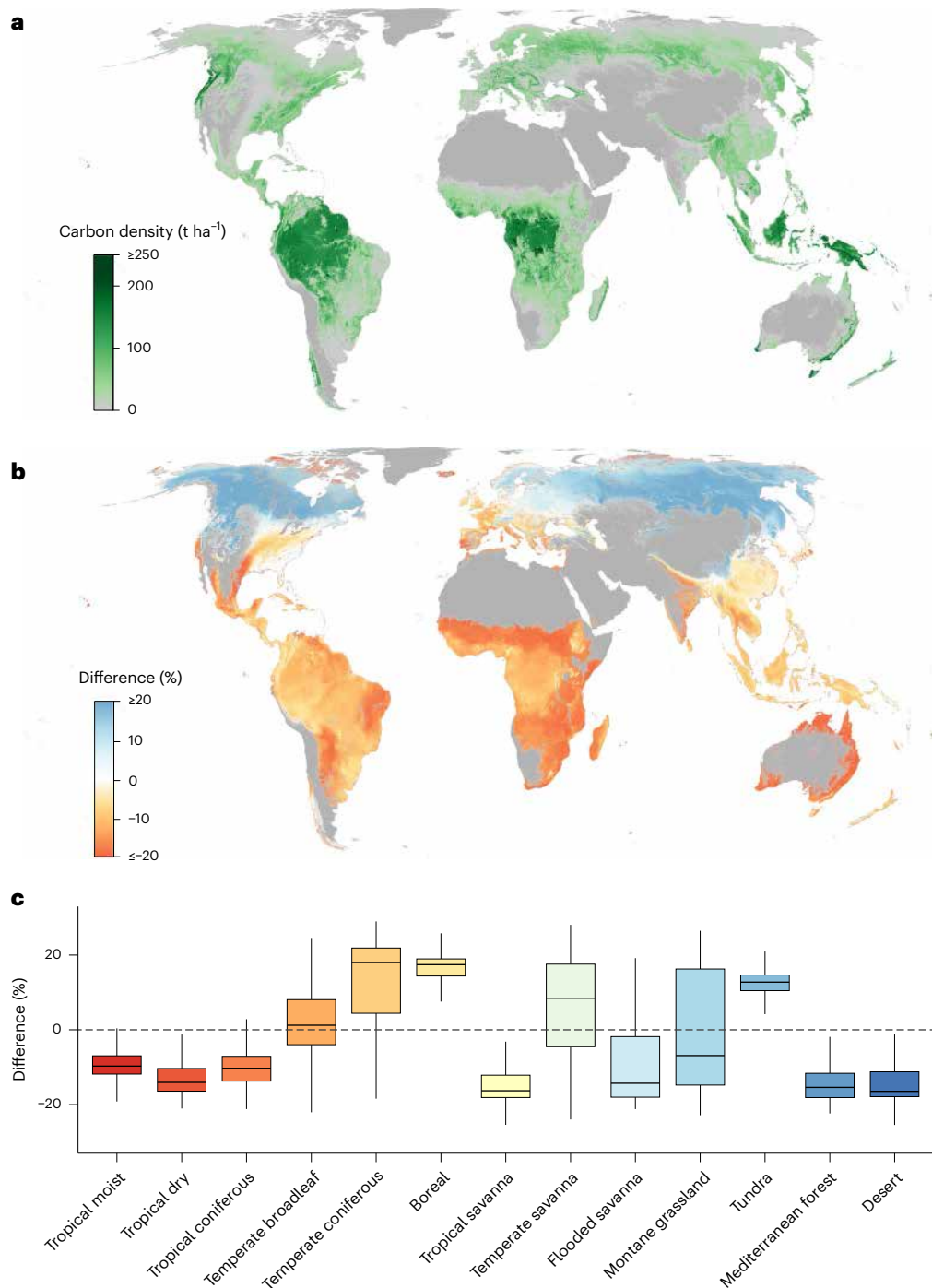
Fig. 5 | Comparison of global living tree biomass distribution using spatially explicit wood density data versus a universal wood density value. a, The global distribution of living tree biomass (in tonnes per hectare), derived by integrating our wood density map with spatially explicit data on living tree volume, root mass fraction and biomass expansion factors. b, Percentage difference in estimated living tree biomass when comparing results derived using the global wood density map (from a ) with estimates using a single, universal
