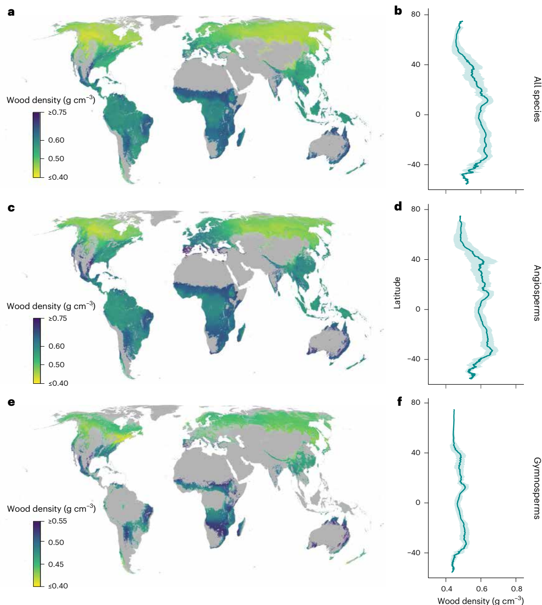
Fig. 3 | Global maps of wood density. a,c,e , Wood density maps for all species (a), angiosperms-only (c) and gymnosperms-only (e). a , The community-level wood density map was derived from an ensemble approach, averaging the global predictions from the 200 best random-forest models. c,e , Angiosperm-only (c) and gymnosperm-only (e) wood density maps were derived from ensemble averaging of the global predictions from the 100 best random-forest models, respectively. b,d,f , Corresponding latitudinal trends in wood density
