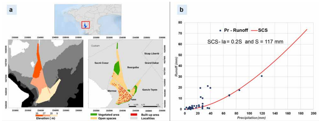
Figure 5. (a) Characteristics of the Fann–Mermoz experimental basin. (b) The relationship between rainfall and runoff (data taken from Bassel, 1996).
