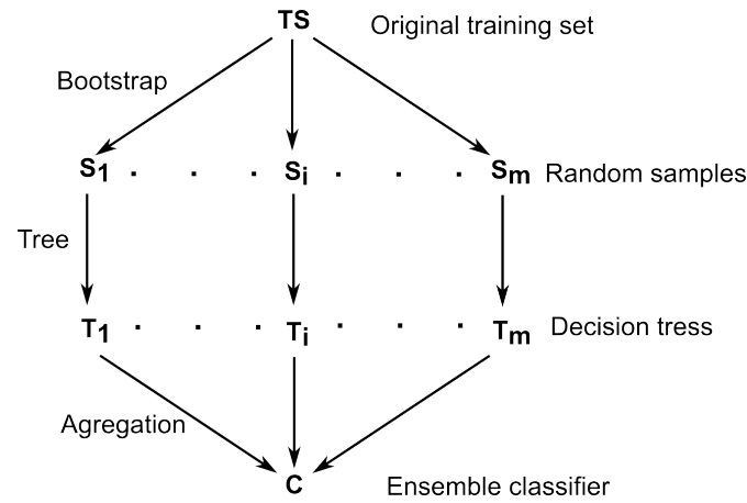
Figure 4. Random Forests principle
