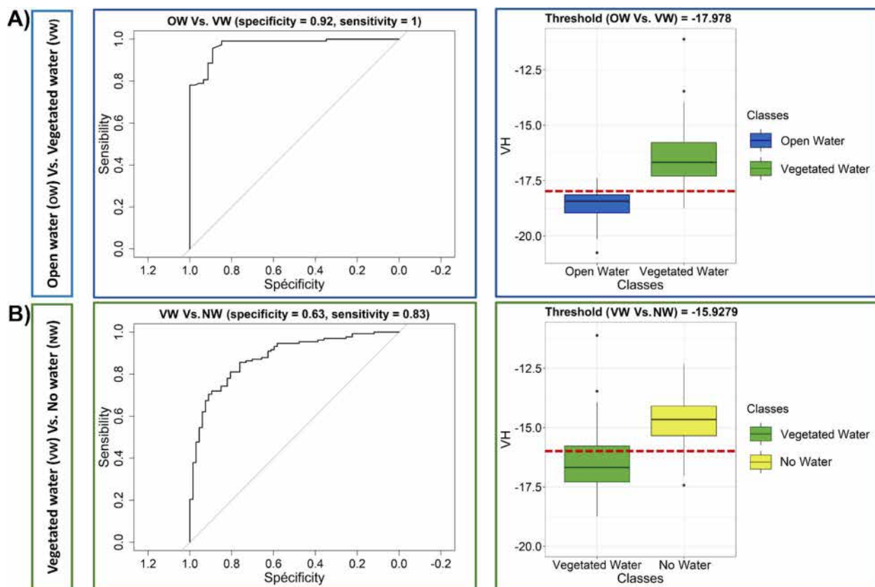
Fig. 3 Result of receiver operating characteristic (ROC) curve analyses on the test dataset and resulting threshold in VH polarizations. a Comparison of ROC Curve between Open water (Positive) and Vegetated water (Negative) of sample rice fields. b Comparison of ROC Curve between Vegetated water (Positive) and No water (Negative) of sample rice fields. Both ROC curve confusion matrices are described in the Results section and (see Additional File 1: Tables S1–S3)
