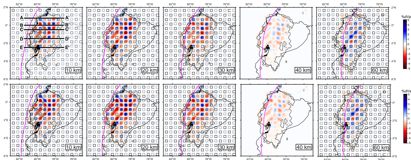
Figure 5. Depth slices through synthetic checkerboard tests. Black squares define the synthetic input anomalies. Dashed lines show input checkers of -5\% V_p (top row) and V_s (bottom row). Solid lines show input checkers of +5\% V_p and V_s . The dark grey contour line encloses nodes within the model with > 5 sampling rays. We note that the 40 km layer does not have any synthetic anomalies within it.
