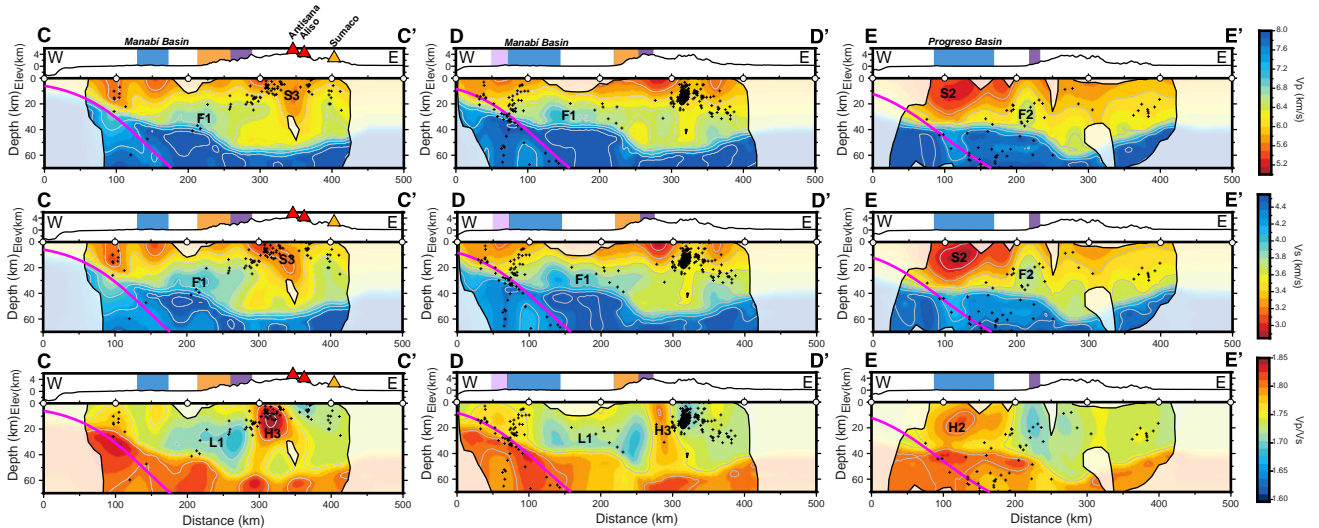
Figure 10. Cross-sections through V_p (top row), V_s (middle row) and V_p/V_s models (bottom row). Each cross-section includes topography above. Behind the topography is plotted major terranes and basins (see Fig. 9 for legend). Black crosses show the hypocentres of earthquakes from this study. Red triangles show the location of Holocene volcanoes within 10 km of the cross-section. The names of each volcano are shown above in the top row.
