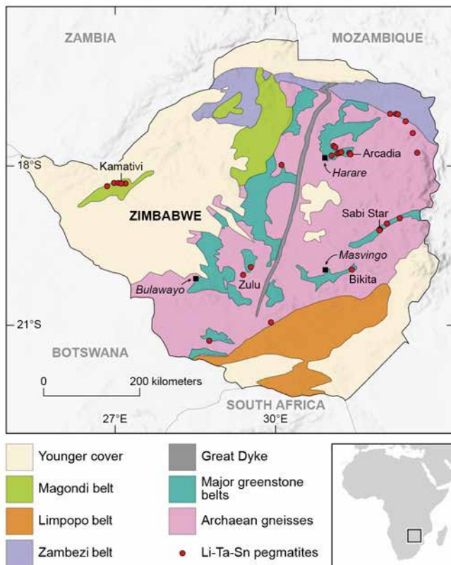
Fig. 4. Simplified geologic map of Zimbabwe after Shaw et al. (2022) with pegmatite locations indicated.
