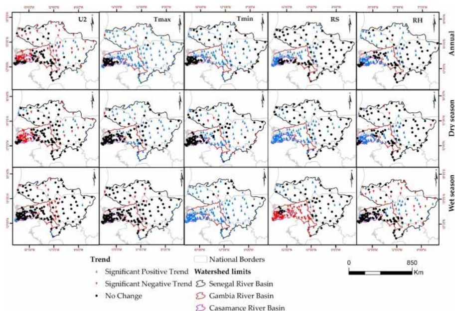
Figure 4. Spatial repartition of the trend of climatic variables on annual and seasonal scale over the period 1984–2019 (RH: relative humidity, T_{\max} : maximum temperature, T_{\min} : minimum temperature, R_S : Solar radiation and U_2 : wind speed).
