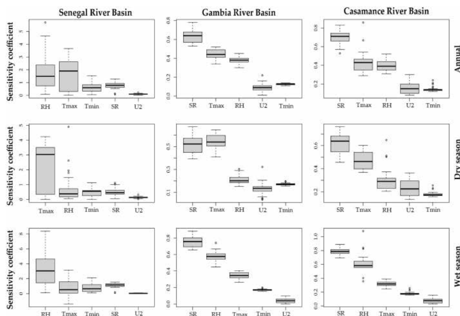
Figure 6. Mean sensitivity coefficient of climatic variables over the period 1984–2019 (RH: relative humidity, T_{\max} : maximum temperature, T_{\min} : minimum temperature, R_s : Solar radiation and U_2 : wind speed).
