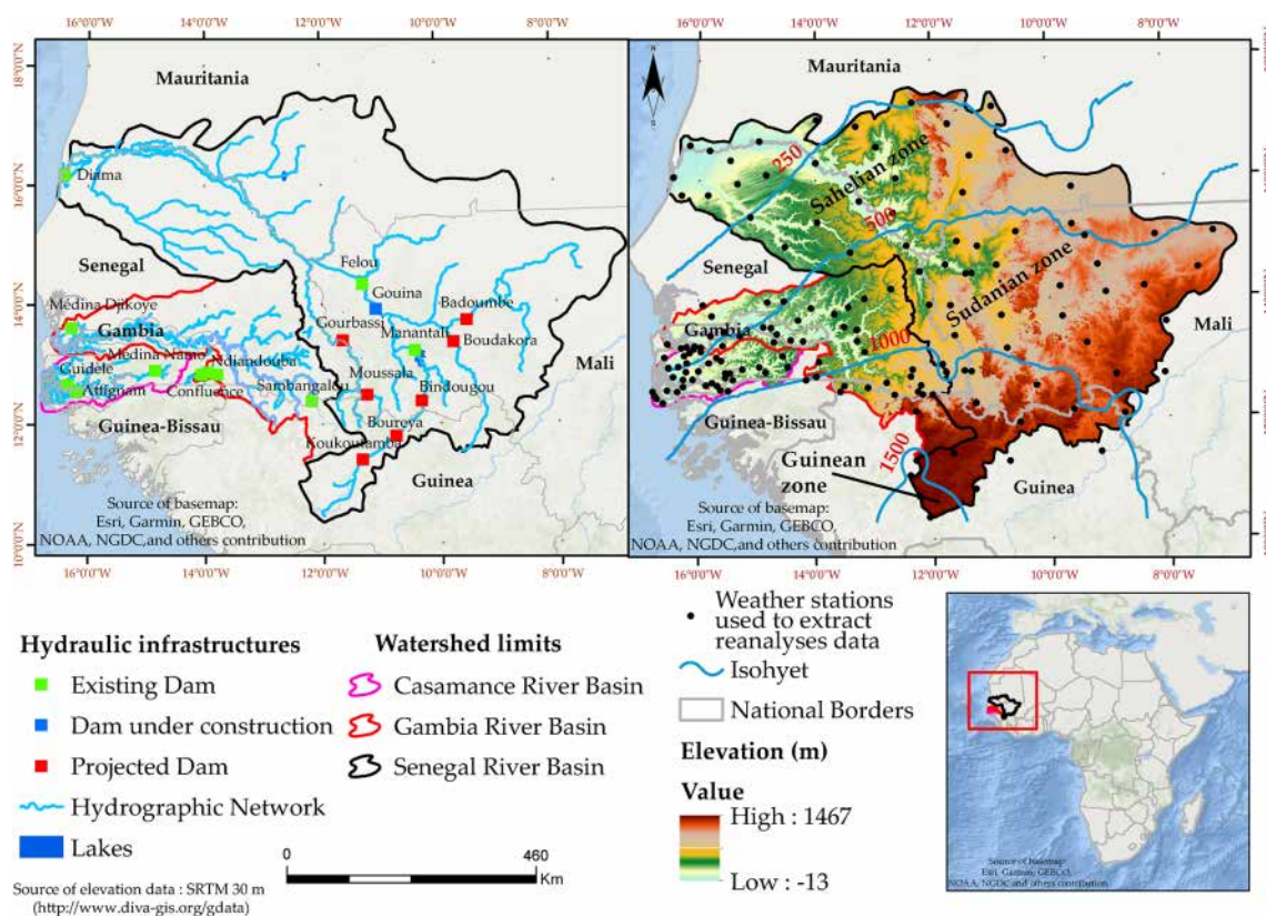
Figure 1. Location of the Senegal hydrosystems, hydraulic infrastructures, climate zones, hydrographic network and weather stations used to extract reanalyses data.
