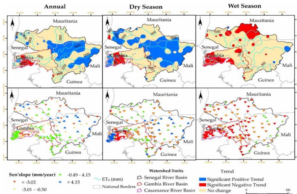
Figure 2. Trend of annual and seasonal reference evapotranspiration over the period 1984–2019.
