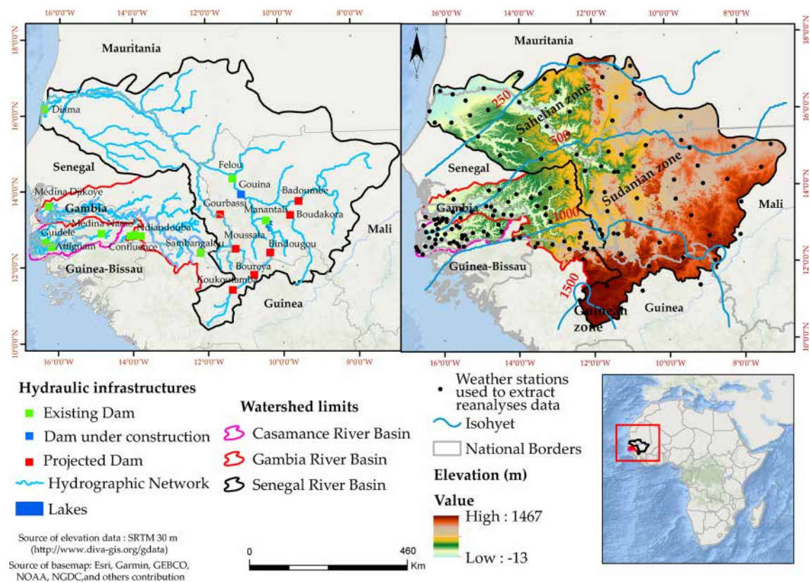
Figure 1. Location of the three Senegalese hydrosystems, hydraulic infrastructures, climate zones, hydrographic network and weather stations used to extract reanalyses data.
