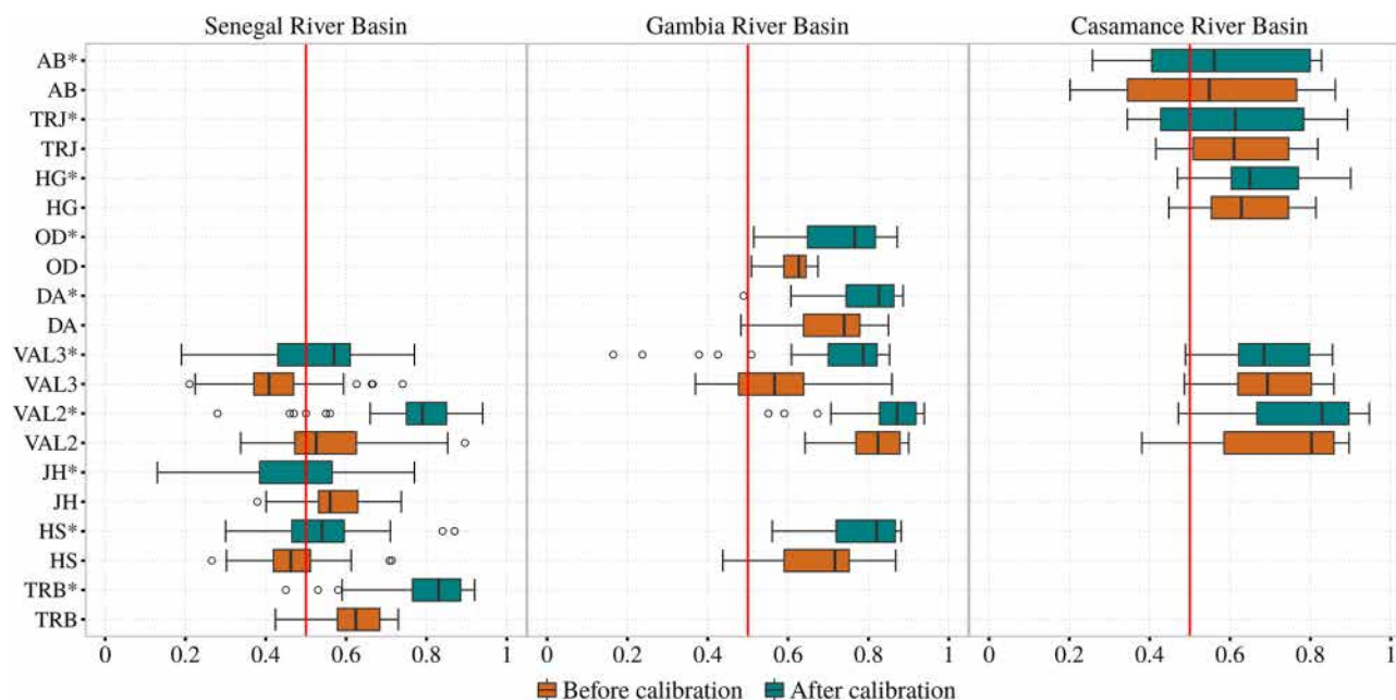
Figure 3. KGE values before and after calibration.
