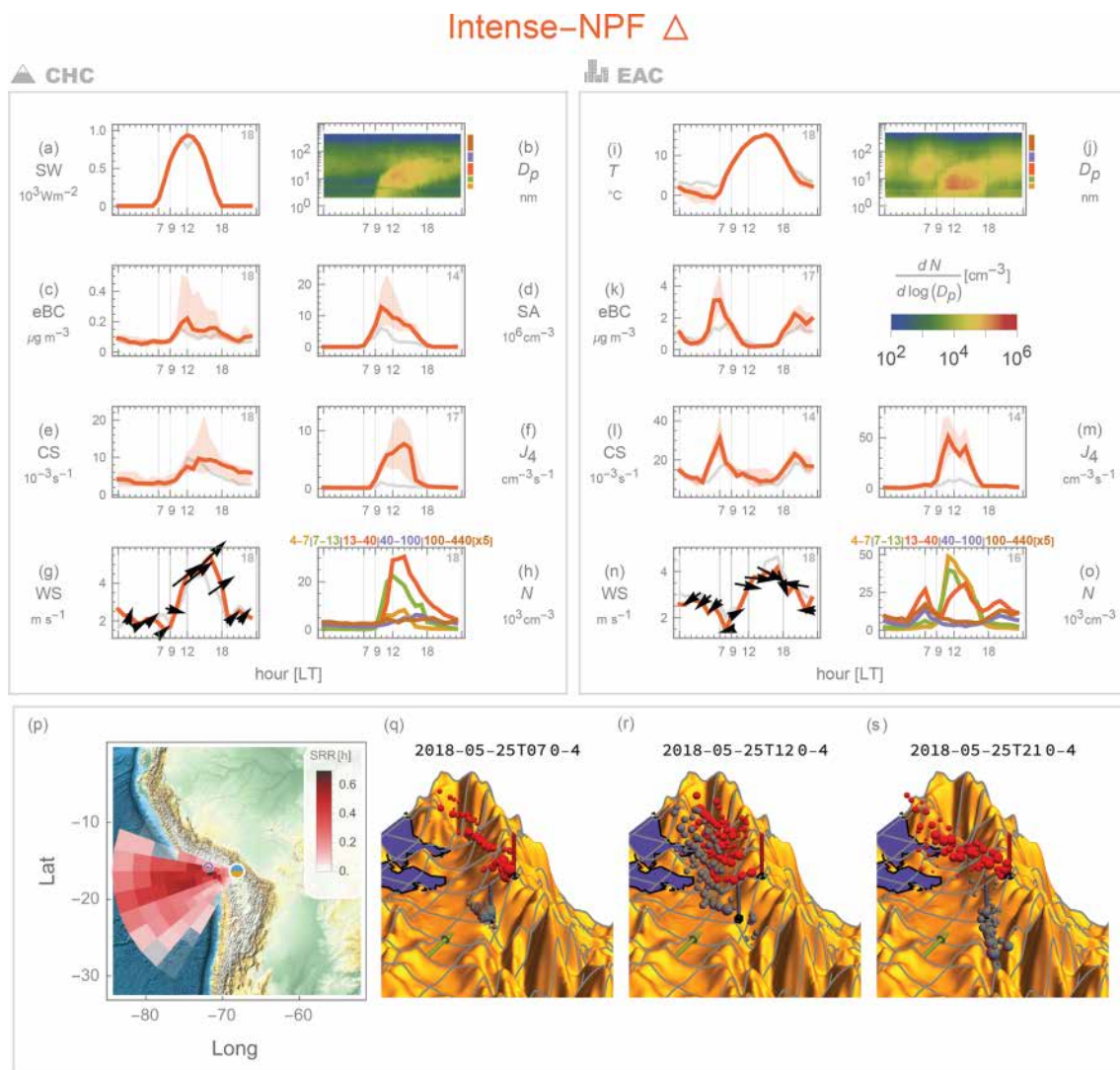
Figure 5. Main characteristics of the Intense-NPF category. Panels (a)–(h) and (i)–(o) provide information on diurnal median values of key variables at CHC and EAC, respectively. The shading shows the inter-quantile range, and the grey line is the median of all categories (shown for comparison). Panels (g) and (n) show the wind speed, and the arrows point to the median direction (up means wind coming from south to north, and right means wind coming from west to east). Panels (h) and (o) show the concentration at different ranges color coded and specified in the legend above. Panel (p) shows the median long-range air mass origins for CHC (source–receptor relationship; SRR). The sky-blue half-disk represents the location of CHC (with EAC in orange close to the same location). The lilac circle marks the location of the Sabancaya volcano. The EAC long-range air mass origin is very similar and is presented in Fig. 9. Panels (q)–(s) depict the short-range ( < 4 h) air mass origins for a representative day at three key hours: 7, 12, and 21 (see Sect. 3 for calculation). The red spheres indicate the location of the air mass arriving at CHC, with their size representing the quantity and/or duration of air tracers in that location. The grey spheres provide the same information but for EAC. The green arrow points north. CHC is denoted by a pyramid with a red stick on top, while EAC is marked with a cube topped by a grey stick. Each grid line is separated by approximately 25 km.
