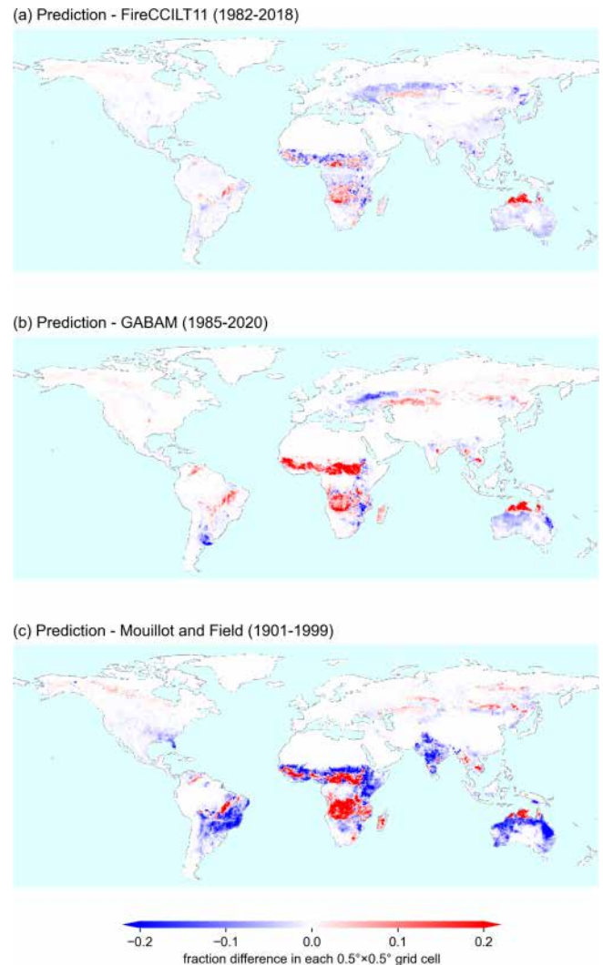
Figure 7. Maps of burned area fraction difference between our predictions and other global burned area datasets. (a) Map of the multi-year average (1982–2018) burned area fraction difference between our predictions and FireCCILT11 (the former minus the latter). (b, c) Same as (a) but using the Global Annual Burned Area Maps (GABAM) (1985–2020) and Mouillot and Field (2005) (1901–1999), respectively. Note that there are several years (1986, 1988, 1990, 1991, 1993, 1994, 1997 and 1999) without available data before 2000 in GABAM.
