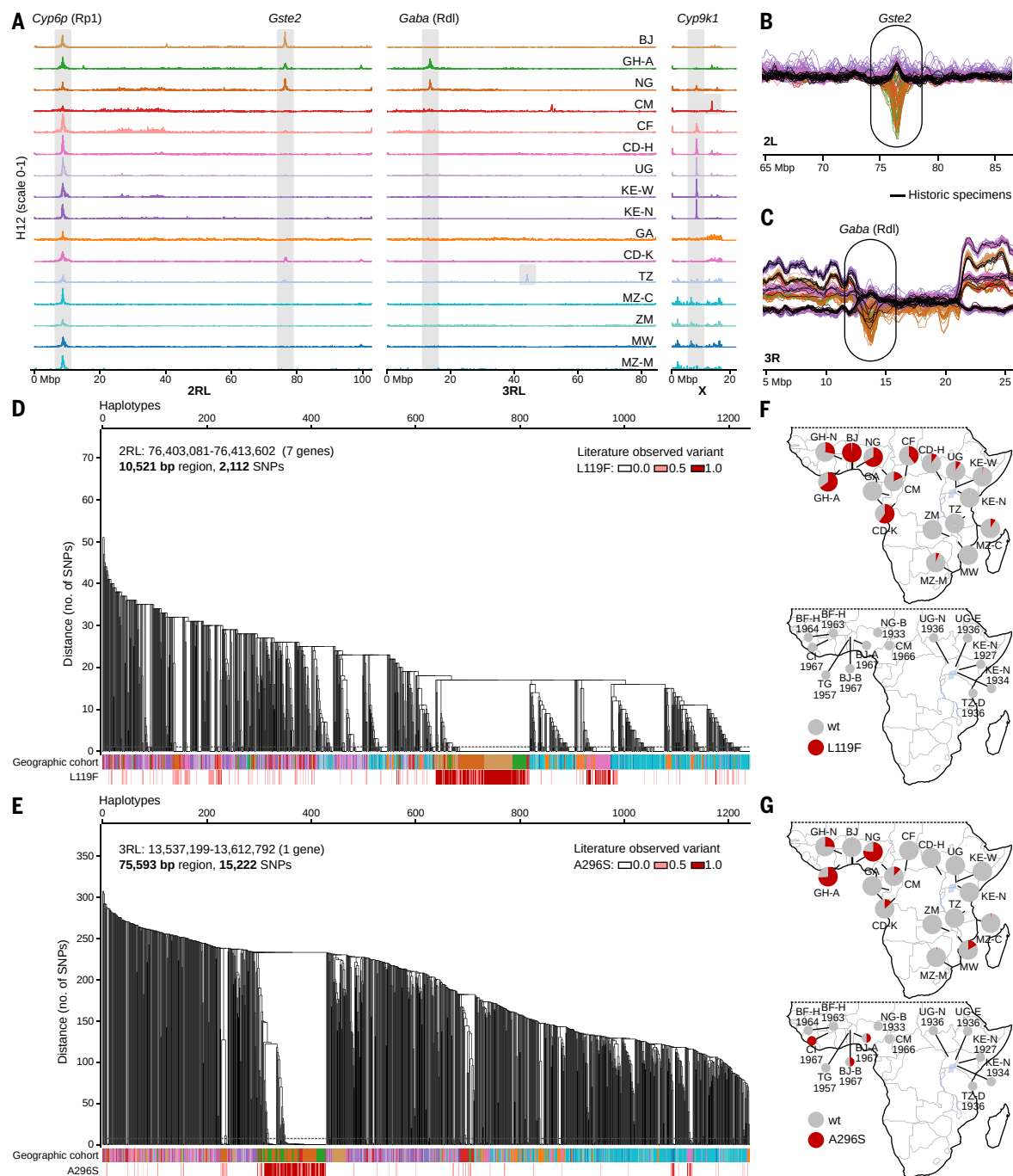
Fig. 3. Selection sweeps and known insecticide resistance variants in Gste2 and Gaba . (A) Genome-wide H12 scans for signals of recent selection. H12 values range from 0 to 1, with higher values indicating excessive haplotype sharing, which is a signature of recent selection. North Ghana was excluded owing to elevated runs of homozygosity, which adds noise and makes H12 values unreliable for detecting genuine selection signals. The y axis runs from 0 to 1 for each cohort, and the x axis shows positions along the genome. Peaks of H12 values \geq 0.4 are highlighted with a gray vertical bar; for peaks where only one cohort reaches this threshold, the bar is restricted to this cohort. (B) Sliding window PCA computed on modern samples and historic samples combined, excluding North Ghana. For visualization purposes, only present-day Equatorial and South Benin cohorts and the historic Equatorial cohort are shown (for full sliding window PCA, see fig. S11D), and the plot is restricted to a 20-Mbp region around the Gste2 gene. Present-day samples show a peak in the Gste2 region (indicated by black ellipse), which is likely a signal of selection, whereas historic samples (shown in black) do not exhibit this signal. (C) Sliding window PCA computed on samples subsetting as in (B), here showing a 20-Mbp region around the Gaba gene. Several historic samples follow the peak seen in present-day samples at the Gaba locus. (D) Haplotype clustering within a region containing seven Gste genes. The dendrogram was obtained by hierarchical clustering of phased haplotypes and used to define haplotype clusters as groups of haplotypes with SNP divergence < 0.0005 (cutoff indicated as dashed horizontal line on the dendrogram). The first bar below the dendrogram shows the population of origin for each haplotype, the second bar shows the genotype for the known Gste2 Leu 119 Phe (L119F) mutation (note that this mutation was filtered out before haplotype phasing, so each haplotype is colored by the genotype of the individual it belongs to; fig. S8A and table S3). (E) Haplotype clustering within the Gaba gene. Same structure as in (D), with the red bar showing the genotype for the rdl Ala 296 Ser (A296S) variant (fig. S8B and table S3). (F) Maps showcasing the frequency of the L119F mutation in present-day (above) and historic (below) sample sets. (G) Maps showcasing the frequency of the rdl A296S mutation in present-day (above) and historic (below) sample sets. Single-letter abbreviations for the amino acid residues referenced throughout this paper are as follows: L, Leu; F, Phe; A, Ala; S, Ser.
