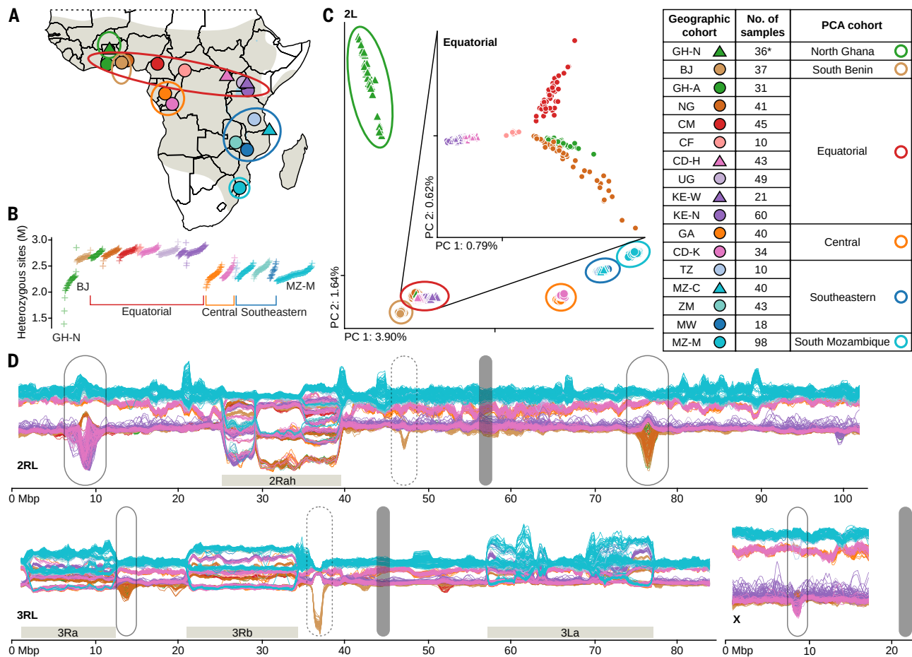
Fig. 1. Population structure of 656 An. funestus specimens collected across Africa. (A) Map showing sequenced individuals from sub-Saharan Africa grouped into 17 geographic cohorts based on their collection location (filled circular and triangular markers) and 6 PCA cohorts consisting of one or more geographic cohorts (open elliptical markers), with the gray shaded area showing the An. funestus range across the continent [adapted from Sinka et al. (1)]. The asterisk represents one sample collected in GH-N that clusters with Equatorial on the PCA and has therefore been removed in analyses using PCA cohorts. (B) Number of heterozygous sites (in millions) per individual, with each cross representing one individual in subset_2 (females only; for subset_1, see fig. S2A) and ordered along the horizontal axis by geographic cohort (color, same order as the legend) and number of heterozygous sites. (C) Projection along the first two PCs computed on chromosome arm 2L, with the percentage of explained variance in the axis labels and ticks denoting the 0 position along each axis. The PCA cohorts are indicated with open elliptical markers. The inset PC plot was computed only on samples from the Equatorial PCA cohort. (D) Sliding window PCA along the genome. Each line corresponds to one individual, and individuals from GH-N were excluded. The genome was split in overlapping windows of approximately 1-Mbp and 200-kbp steps, a PCA was performed for each window, PC1 values are plotted along the y axis, and the window centers in genomic coordinates are plotted along the x axis. (the corresponding plot displaying the PC2 values for the same windows is shown in fig. S7A). Inversion regions are indicated by horizontal gray bars, centromeres are indicated by vertical grey bars, and lined ellipses indicate regions of divergence across several cohorts (Fig. 3 and figs. S8 to S10), whereas the two dotted ellipses showcase divergence specific to the South Benin PCA cohort (fig. S5, B and C). GH-N, Ghana Northern Region; BJ, Benin; GH-A, Ghana Ashanti; NG, Nigeria; CM, Cameroon; CF, Central African Republic; CD-H, Democratic Republic of the Congo, Haut-Uélé; UG, Uganda; KE-W, Kenya Western Province; KE-N, Kenya Nyanza; GA, Gabon; CD-K, Democratic Republic of the Congo Kinshasa; TZ, Tanzania; MZ-C, Mozambique Cabo Delgado; ZM, Zambia; MW, Malawi; MZ-M, Mozambique Maputo.
