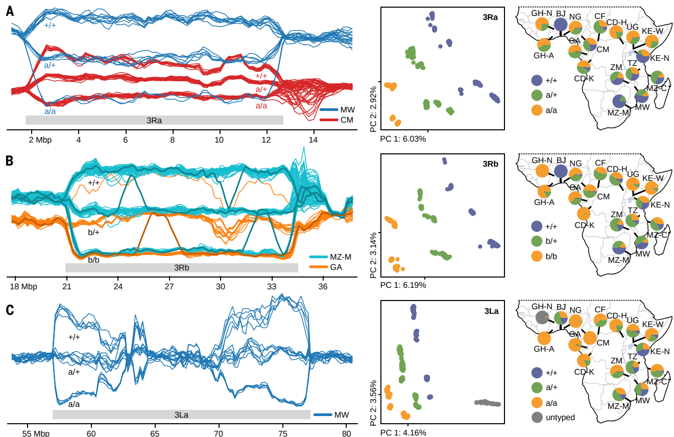
Fig. 2. Segregating inversions on chromosome 3. Sliding window PCAs (left) were computed on all samples except North Ghana. For visualization purposes, only a subset of samples is shown for each sliding window PCA. (A) (Left) Sliding window PCA showing CM (red) and MW (blue) samples on the 3Ra inversion region; window centers are plotted in mega-base pairs along the x axis, and PC1 values for each individual, along the y axis. The different karyotypes are visible as three different horizontal trajectories: from top to bottom, 3R+/, 3Ra/+, and 3Ra/a. All three karyotypes are present in both cohorts, and because PC1 captures a signal that is a combination of the inversion and geographic population structure, the upper and middle trajectories (3R+/+ and 3Ra/+, respectively) do not overlap for the different cohorts; see fig. S7D. (Middle) Projection along the first two PCs computed on the entire inversion region using all samples; samples are colored by inversion karyotype. (Right) Map of karyotype frequencies per geographic cohort. (B) (Left) Sliding window PCA on the 3Rb inversion region displaying GA (orange) and MZ-M (cyan). Several samples change trajectory for part of the inversion region (indicated by thicker, darker lines); these samples appear to be the product of double recombination, and they locally exhibit a different karyotype than they have for the rest of the inversion (see fig. S7E and supplementary materials). The middle and right panels are the same as in (A) but for the 3Rb inversion. (C) Sliding window PCA displaying MW on the 3La inversion region, showing a strong separation of karyotypes near the breakpoints, but the signal decays toward the inversion center (fig. S7B). The middle and right panels are the same as in (A) but for the 3La inversion.
