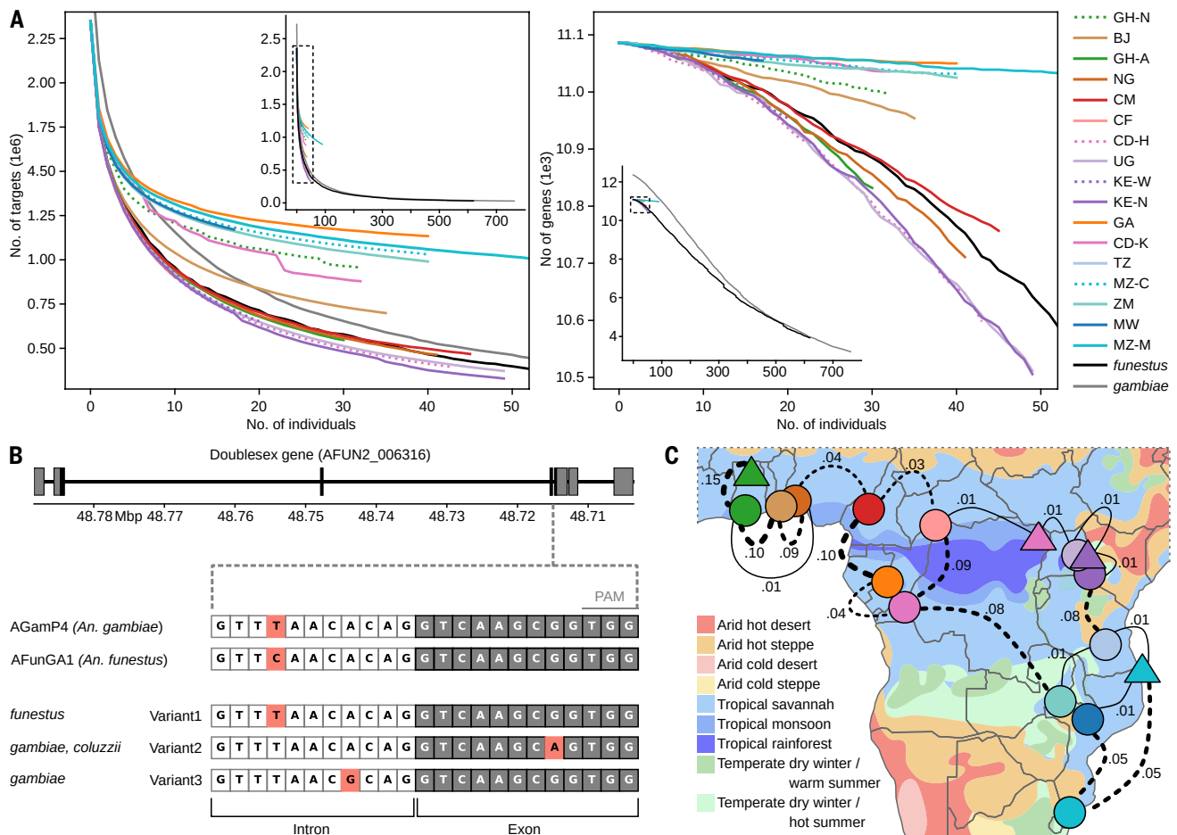
Fig. 4. Challenges for vector control. (A) Cumulative number of gene drive targets (left) and number of genes containing gene drive targets (right) per geographic cohort as well as all subset_2 individuals ( funestus ) and An. gambiae and An. coluzzii individuals from Ag1000G phase 1 (16) ( gambiae ). The insets are zoomed-out versions of the main plots, showing the results for the fully explored datasets; the dashed boxes in the insets indicate the zoomed-in areas shown in the main plots. (B) Sequence variation in the dsx gene drive target on chromosome arm 2R. The dsx gene drive target is located at the boundary of intron 4 and exon 5 of the female-specific isoform. At the top, the seven exons of the female-specific isoform are depicted as boxes on the AGamP4 reference genome; the coding sequence is shown in black, and untranslated exonic regions (UTRs) are shown in grey. The target sequence is shown below; nucleotides in white boxes are located in intron 4, and nucleotides in gray boxes are located in exon 5. The last three nucleotides constitute the PAM. The AgamP4 ( An. gambiae ) and AfunGA1 ( An. funestus ) reference genomes differ at the fourth base of the target sequence (highlighted in pink) in the intronic region. Variant 1 was found at very low frequencies in two cohorts from this study, variant 2 was found at low to intermediate frequencies in four cohorts of An. gambiae and An. coluzzii , and variant 3 was found at very low frequency in one cohort of An. gambiae (see supplementary materials). (C) Map showing F_{ST} for neighboring populations. F_{ST} was calculated on all accessible sites on the 2L chromosome arm. F_{ST} > 0.01 lines are dotted and become thicker as F_{ST} becomes higher. The background of the map is colored by the Köppen-Geiger climate classification, adapted from Beck et al. (56).
