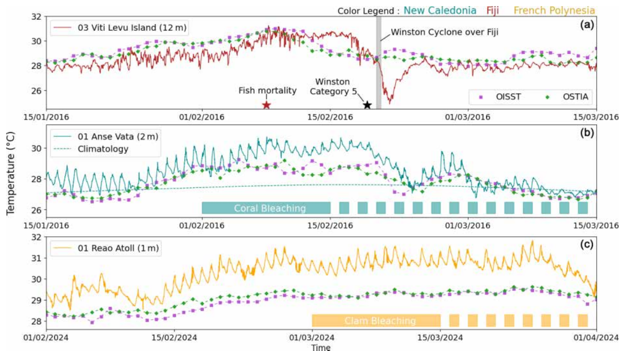
Figure 5. (a) Temperature time series during austral summer 2016 at the Viti Levu Island 03 station (Fiji, depth of 12 m, red line). (b) Temperature time series during austral summer 2016 at the Anse Vata station (New Caledonia, depth of 2 m, dark cyan line). (c) Temperature time series at Reao 01 station (Reao Atoll lagoon, French Polynesia, depth of 1 m, orange line). Daily sea surface temperature from Satellite products are plotted in purple for OISST V2 and green for OSTIA. Dates of the triggered ecosystem impacts are displayed on each subplot (red star for fish mortality in Fiji, dark-cyan bar for coral bleaching in New Caledonia, and orange bar for clam bleaching in French Polynesia). Dotted lines indicate that impacts on coral and clams have continued over time (with no precise end date to give).
