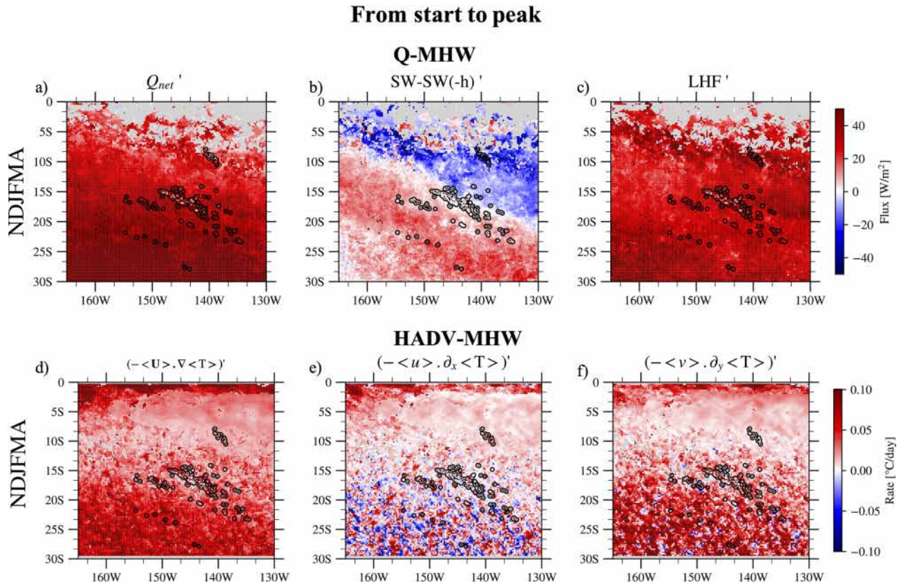
Figure 7. Composites of the net air–sea heat flux (and its dominant components: SW–SW(– h ) and LHF) for Q -MHWs and of the horizontal-advection term (and its decomposition into zonal and meridional components) for HADV-MHWs, for events peaking in the warm season (NDJFMA), averaged over the onset-to-peak period (cf. Sect. 2.2.3). Panels (a)–(c) show Q -MHW composites of (a) net air–sea heat flux Q_{\text{net}} (b) the net shortwave flux stored in the mixed-layer (SW – SW(– h )), and (c) LHF anomalies. Panels (d)–(f) show HADV-MHW composites of (d) horizontal advection anomalies and its (e) zonal and (f) meridional components. In each panel, the composite corresponds to the averaged across all MHWs of the corresponding type ( Q -MHW or HADV-MHW) detected at each grid point.
