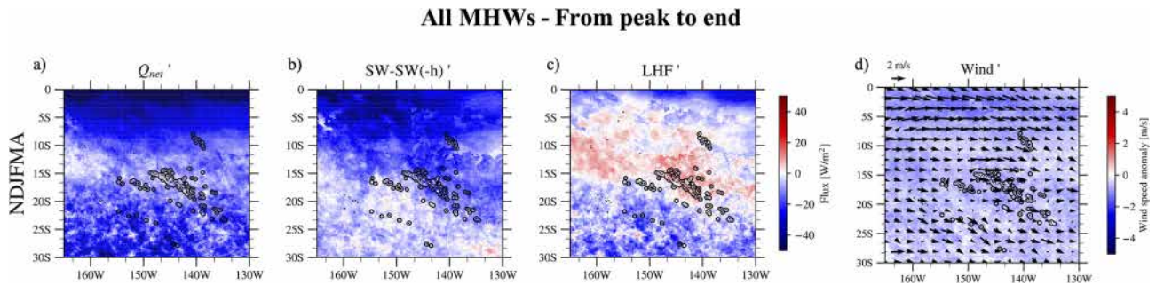
Figure 9. Composites of the net air–sea heat flux (and its dominant components) as well as surface wind anomalies averaged over the decay period i.e. from peak to end (cf. Methods) for all MHWs peaking in austral summer. Panels (a)–(c) show MHW composites of (a) net air–sea heat flux Q_{\text{net}} (b) the net shortwave flux in the mixed-layer ( \text{SW} - \text{SW}(-h) ), and (c) LHF anomalies. In each panel, the composite is averaged across all MHWs (without distinguishing by type as done during the onset period) detected at each grid point.
